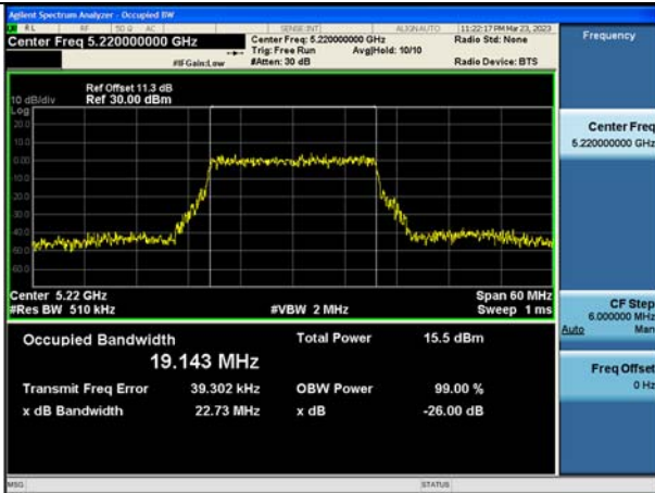
Test Mode:802.11ax HE20 5220MHz Chain1
