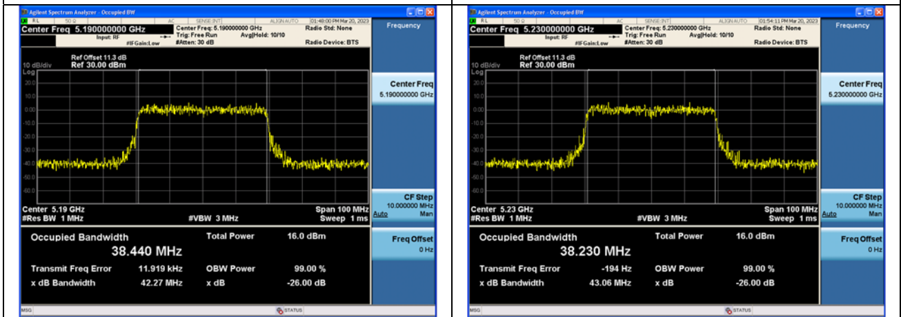
Test Mode:802.11ax HE40 5190MHz Chain1
