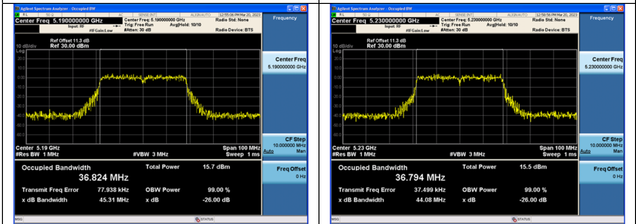
Test Mode:802.11ac VHT40 5190MHz Chain1
