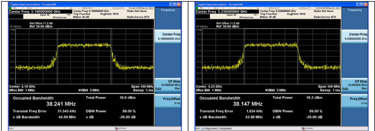
Test Mode:802.11ax HE40 5190MHz Chain0
