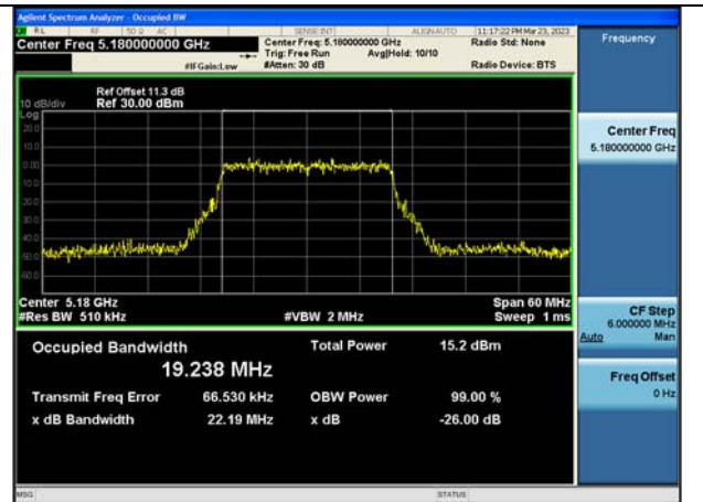
Test Mode:802.11ax HE20 5180MHz Chain1
