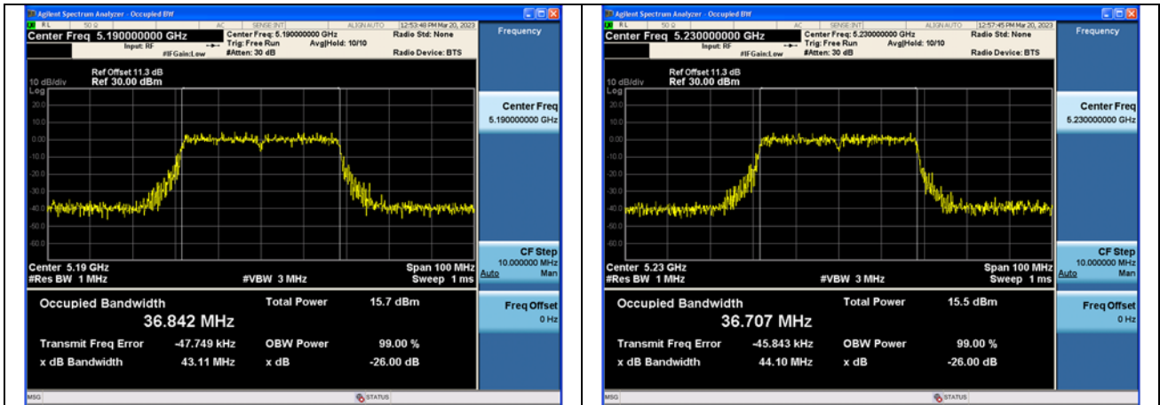
Test Mode:802.11ac VHT40 5190MHz Chain0
