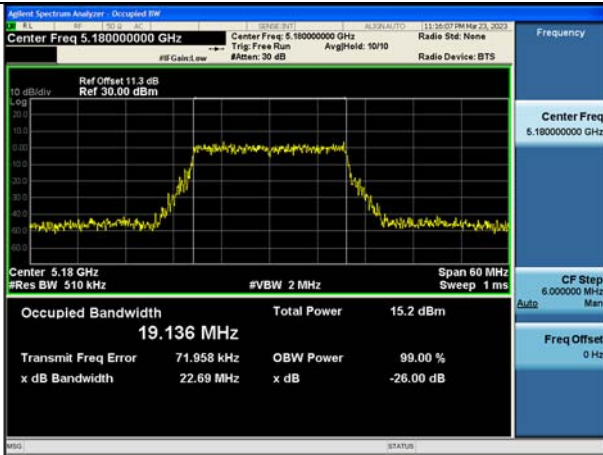
Test Mode:802.11ax HE20 5180MHz Chain0
