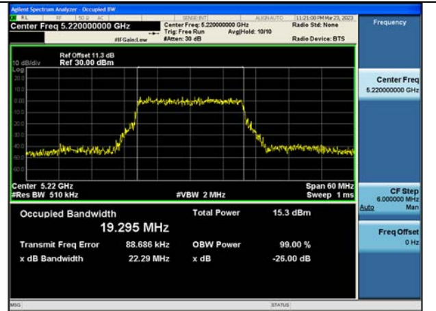
Test Mode:802.11ax HE20 5220MHz Chain0
