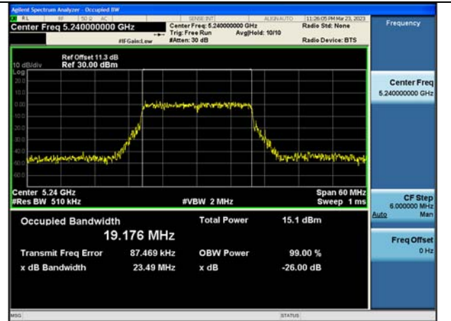
Test Mode:802.11ax HE20 5240MHz Chain1
