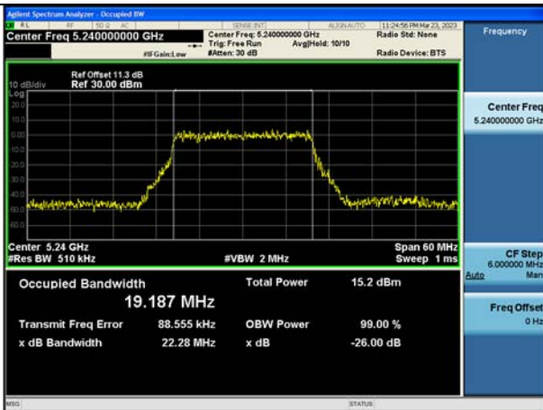
Test Mode:802.11ax HE20 5240MHz Chain0
