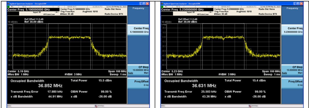
Test Mode:802.11n HT40 5190MHz Chain0
