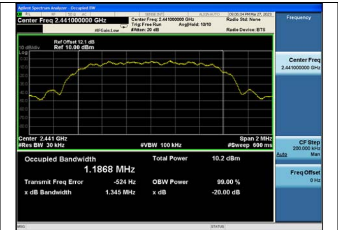
Test Mode: \pi/4 DQPSK(2DH5) 2441MHz
