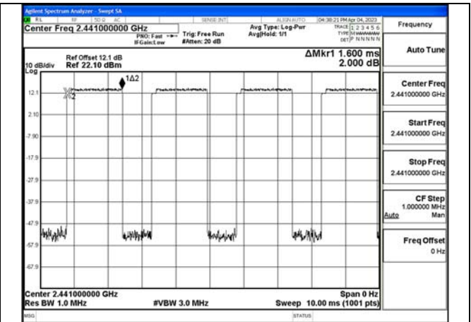
Test Mode: \pi/4 DQPSK(2DH3) 2441MHz
