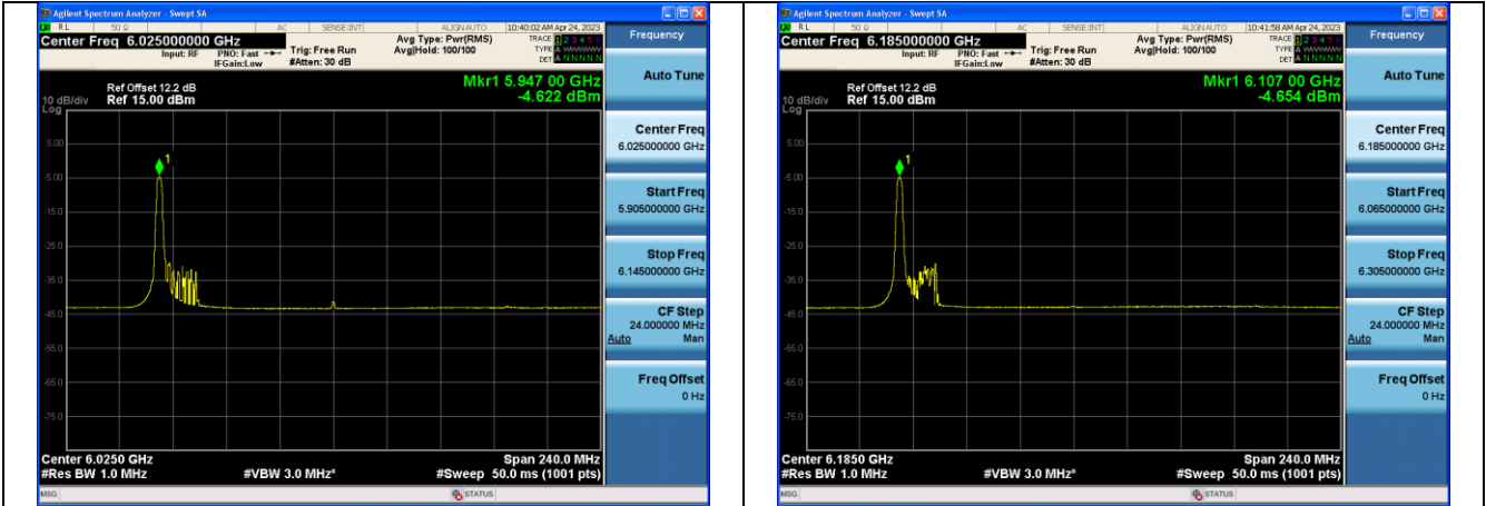
Mode:802.11ax HE160 Tone:26T Frequency:6025MHz Chain0
