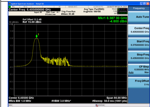
Mode:802.11 ax HE40 Tone:26T Frequency:6405MHz Chain0
