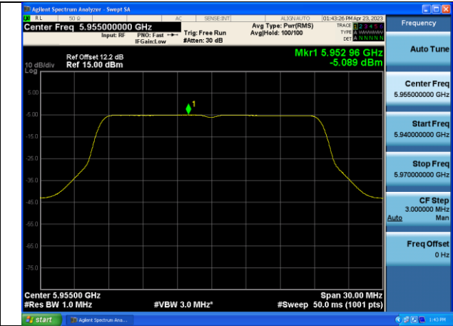
Mode:802.11ax HE20 Tone:242T Frequency:5955MHz Chain1
