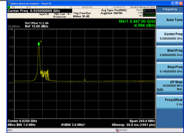
Mode:802.11ax HE160 Tone:26T Frequency:6025MHz Chain1
