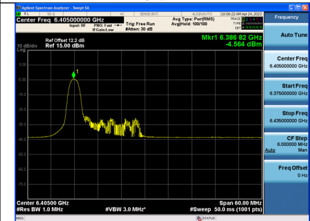
Mode:802.11 ax HE40 Tone:26T Frequency:6405MHz Chain1
