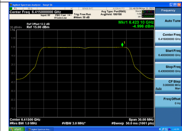
Mode:802.11ax HE20 Tone:242T Frequency:6415MHz Chain1
