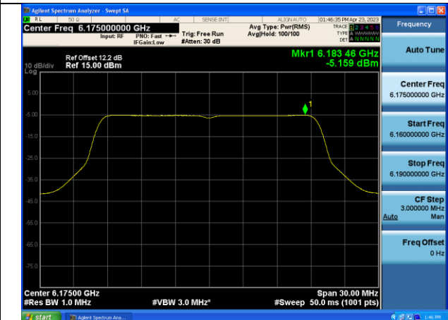
Mode:802.11ax HE20 Tone:242T Frequency:6175MHz Chain0
