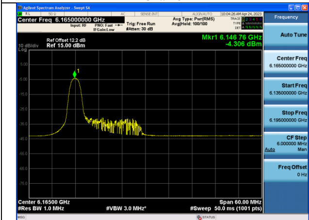
Mode:802.11 ax HE40 Tone:26T Frequency:6165MHz Chain1
