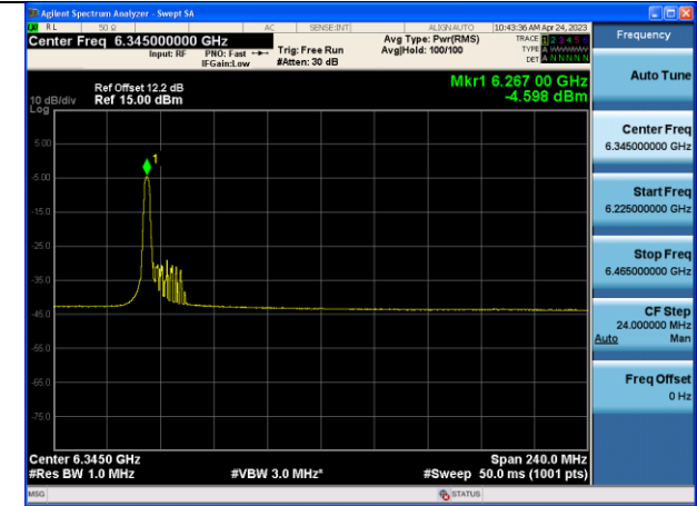
Mode:802.11ax HE160 Tone:26T Frequency:6345MHz Chain1
