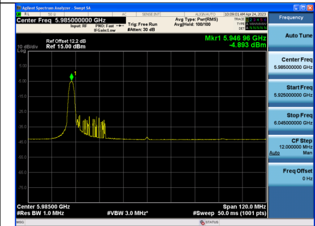
Mode:802.11 ax HE80 Tone:26T Frequency:5985MHz Chain1
