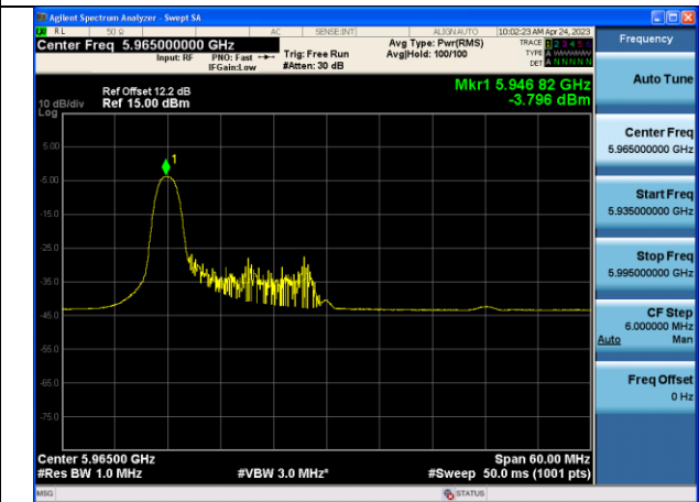
Mode:802.11 ax HE40 Tone:26T Frequency:5965MHz Chain1
