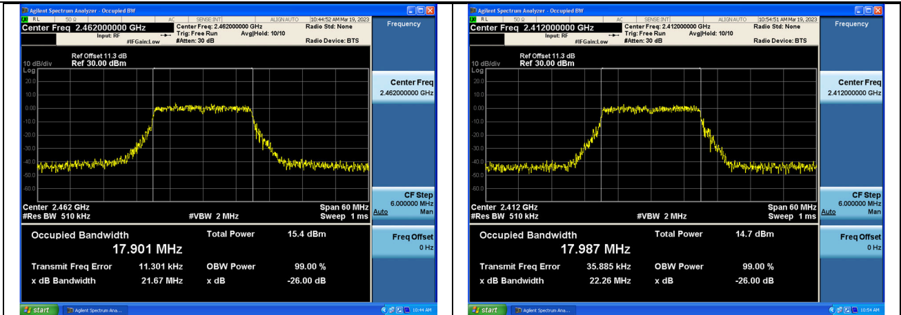
Test Mode:802.11x HE20 2462MHz Chain0
