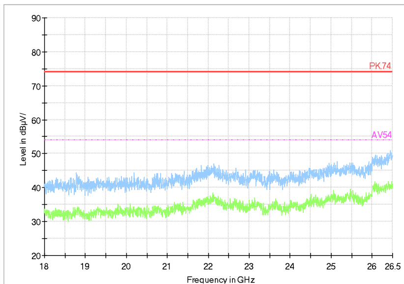
Pic8. Radiated emission (18GHz – 26GHz)
