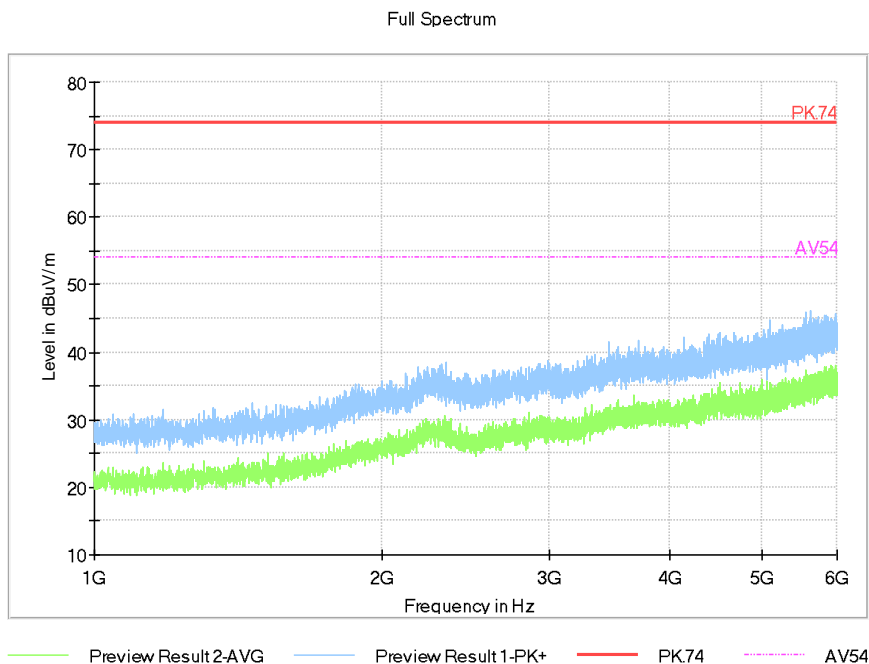
Pic6. Radiated emission (1GHz – 6GHz)
