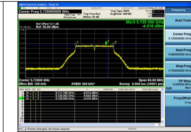
Test Mode:802.11a 5720MHz Chain1 NII2C
