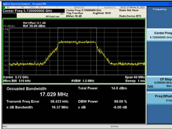
Test Mode:802.11a 5720MHz Chain0 NII2C
