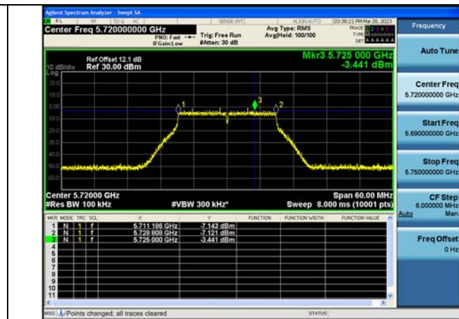
Test Mode:802.11n HT20 5720MHz Chain1 NII2C
