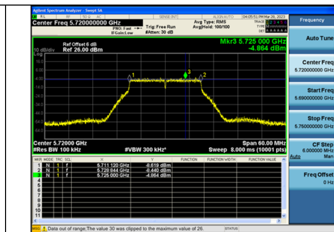
Test Mode:802.11ac VHT20 5720MHz Chain1 NII2C
