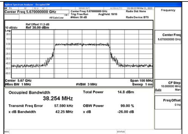
Test Mode:802.11ax HE40 5670MHz Chain1
