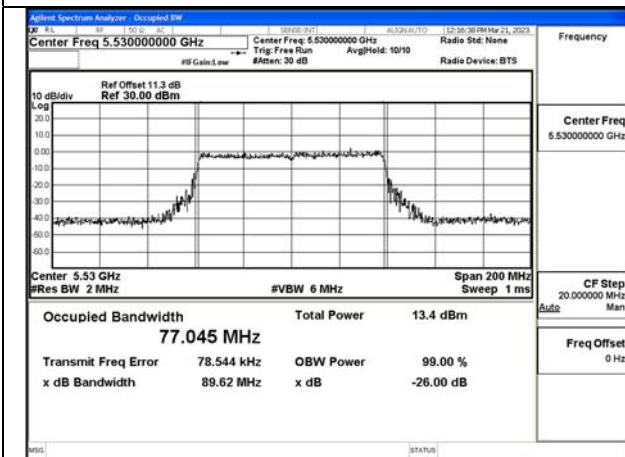
Test Mode:802.11ac VHT80 5530MHz Chain1
