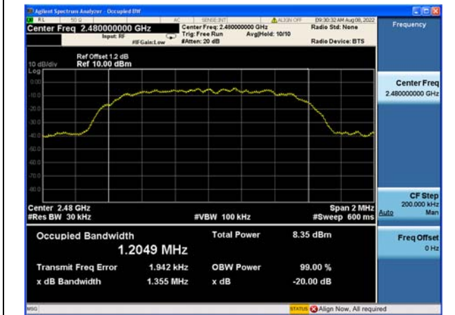
Modulation: 8DPSK 2480MHz
