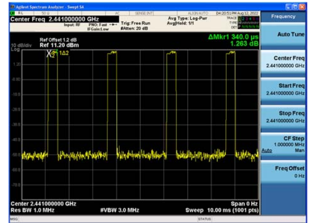
Modulation: 8DPSK 3DH3 2441MHz
