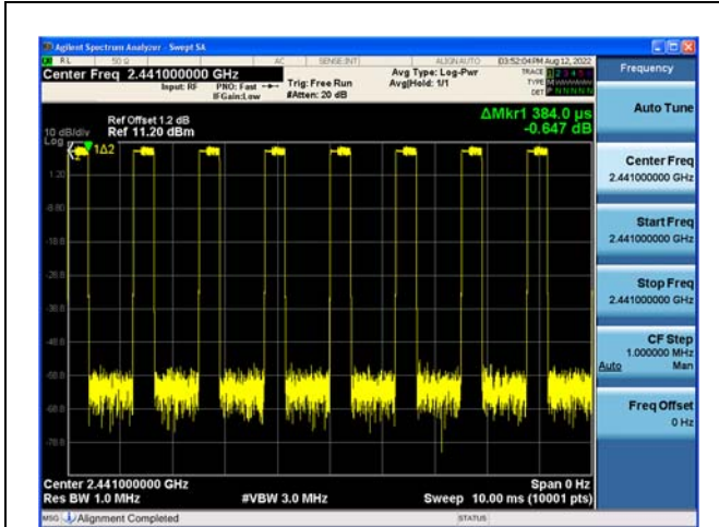
Modulation: \pi/4 DQPSK 2DH1 2441MHz
