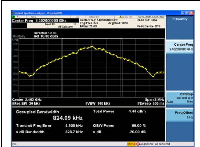
Modulation: GFSK 2402MHz
