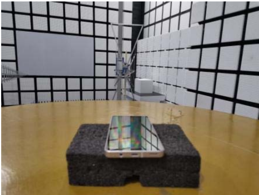
>1GHz
