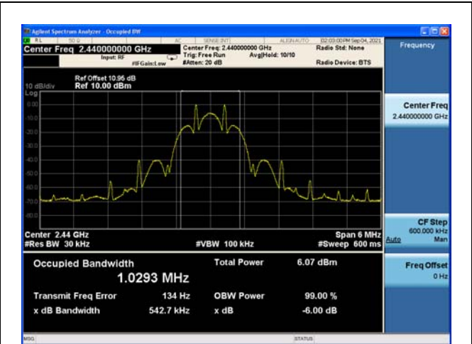
Modulation: Coded 250K 2440MHz
