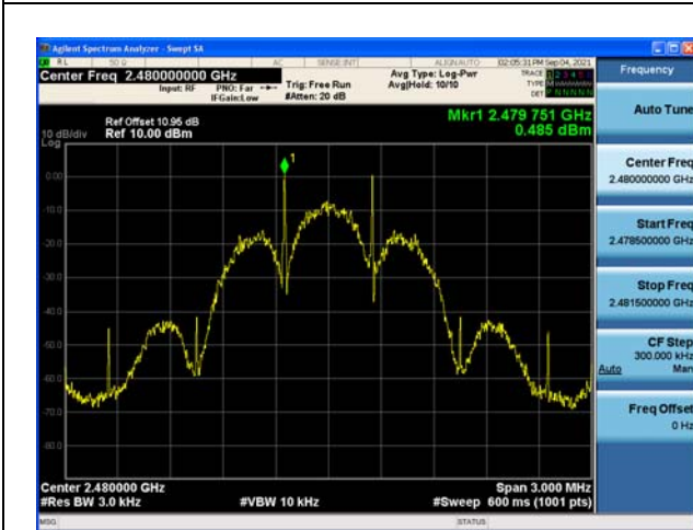
Modulation: Coded 250K 2480MHz
