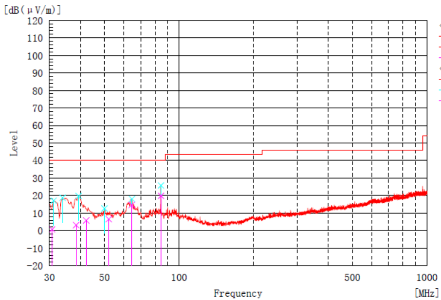
Frequency Range: 30MHz-1000 MHz
