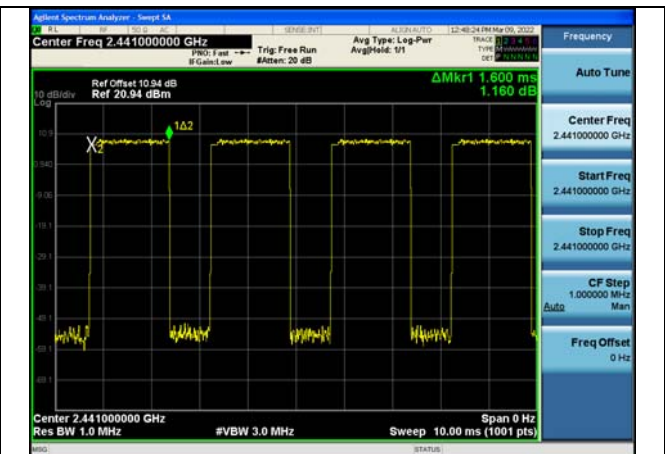
Test Mode:8DPSK(3DH3) 2441MHz
