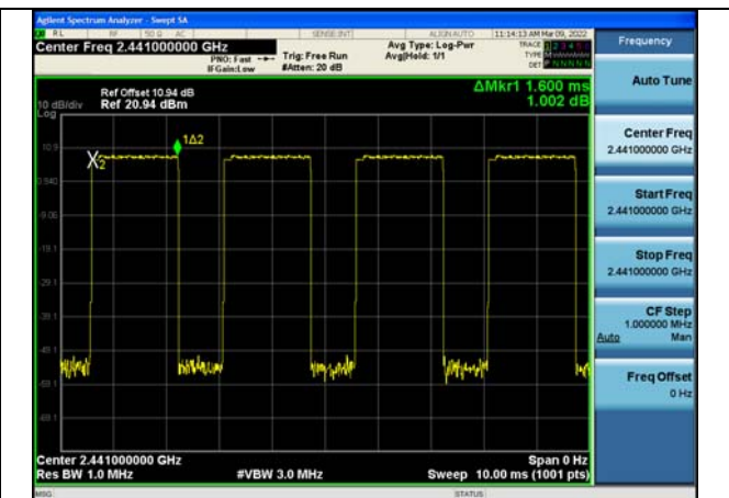
Test Mode:π/4DQPSK(2DH3) 2441MHz
