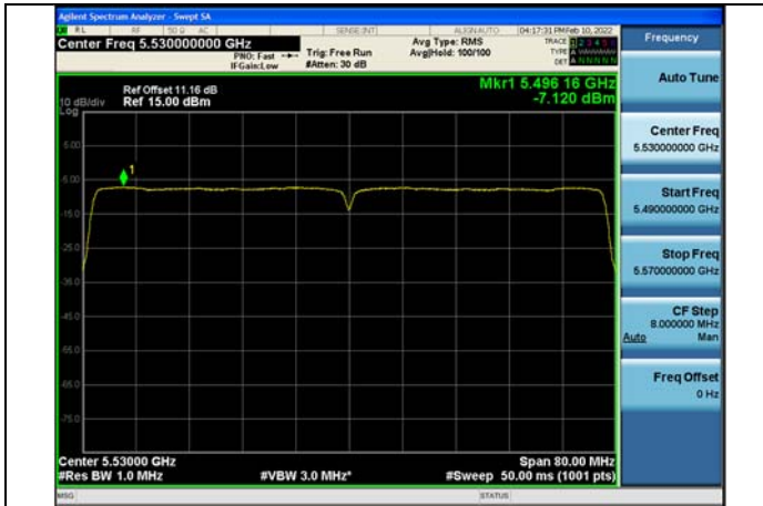
Test Mode:802.11ac VHT80 5530MHz Chain0
