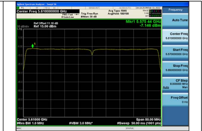
Test Mode:802.11ac VHT80 5610MHz Chain0
