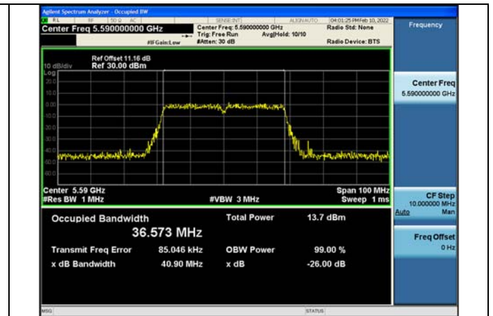
Test Mode:802.11n HT40 5590MHz Chain0
