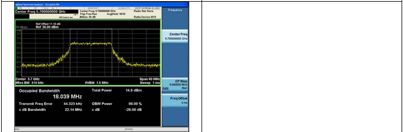
Test Mode:802.11n HT20 5700MHz Chain0
