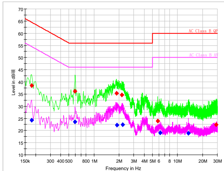
L+N Line
