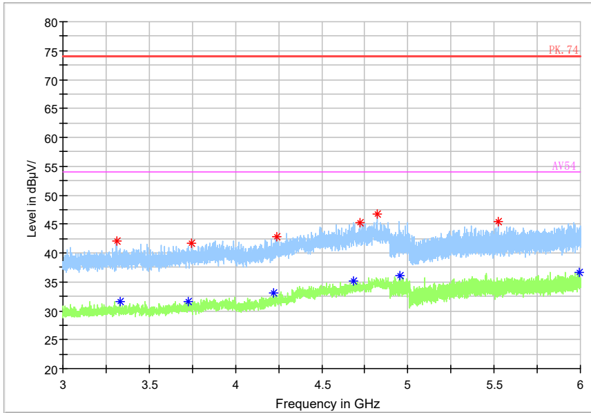
Frequency Range: 3GHz-6GHz Detector: Av mode and PK mode Modulation type: GFSK (LE 2M)
