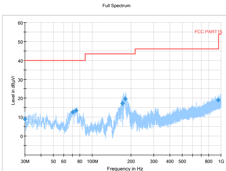
Pic11. Radiated emission (30MHz – 1GHz)
