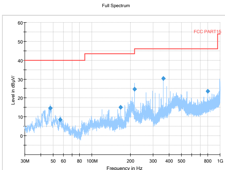
Pic15. Radiated emission (30MHz – 1GHz)
