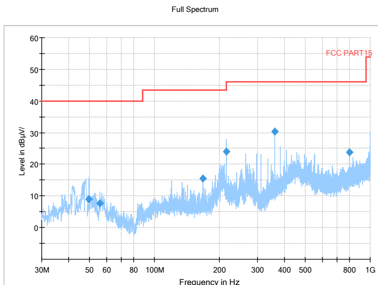
Pic19. Radiated emission (30MHz – 1GHz)
