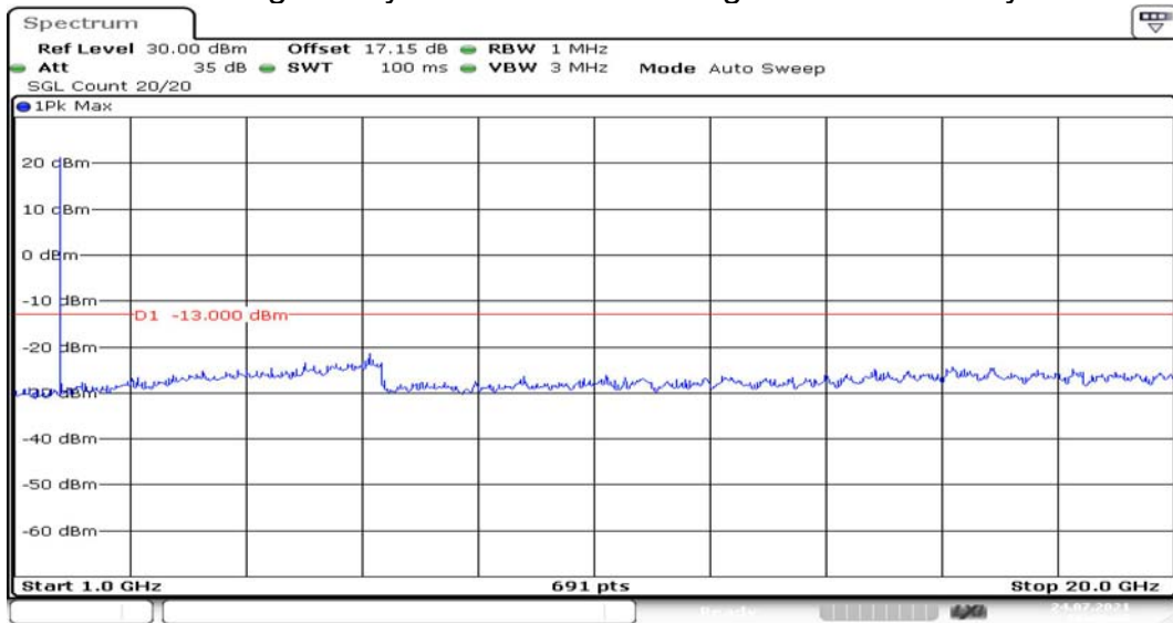
Channel 1412 1GHz~20GHz(dBm)
