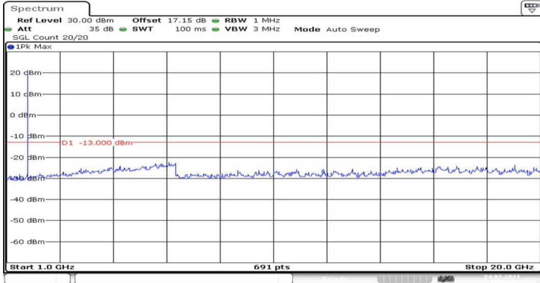
Channel 1412 1GHz~20GHz(dBm)
