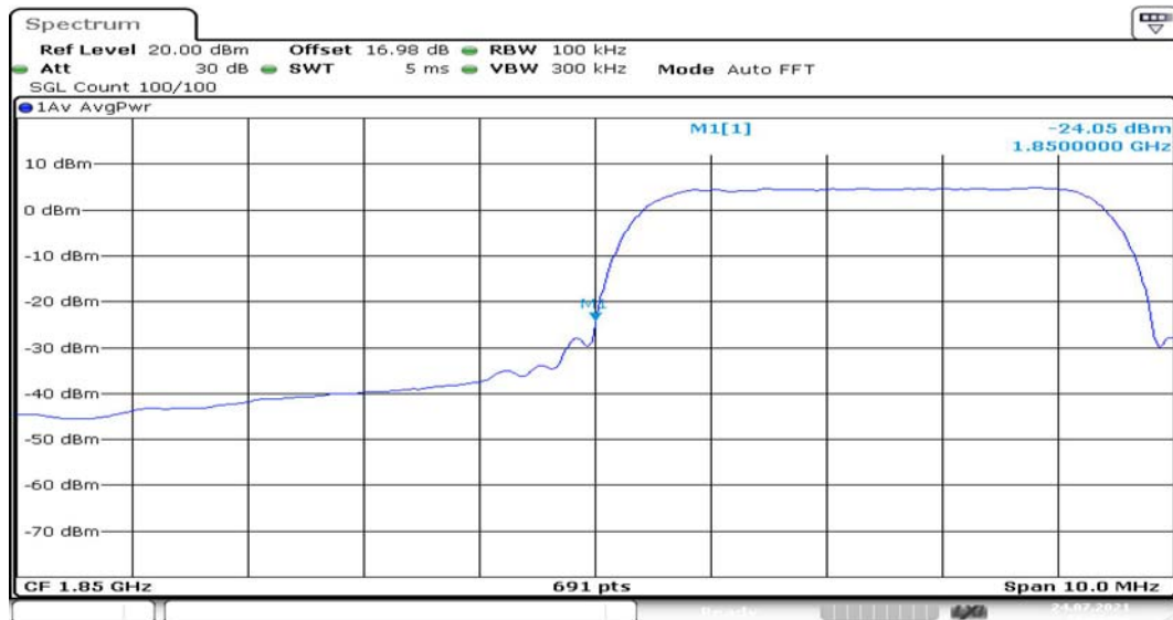
Channel 9262
