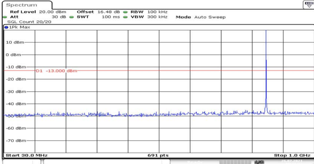
Channel 189 30MHz~1GHz(dBm)
