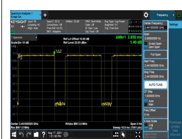
Modulation: 8DPSK DH5 2441MHz
