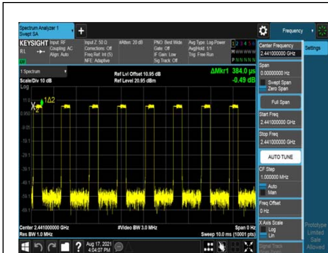
Modulation: \pi/4 DQPSK DH1 2441MHz
