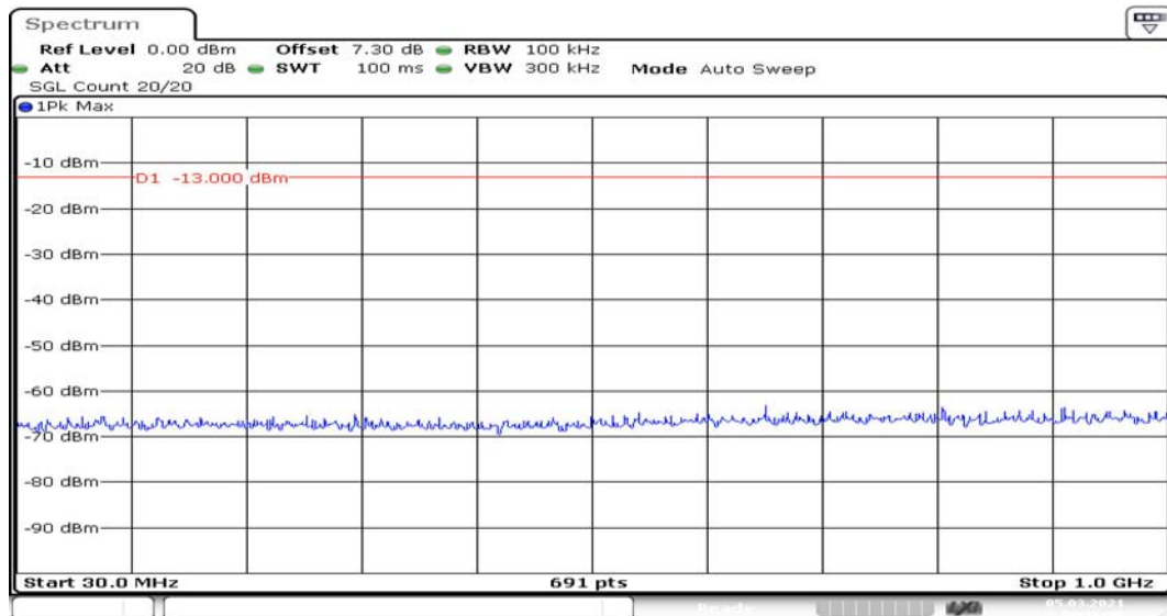
Channel 1412 30MHz~1GHz(dBm)
