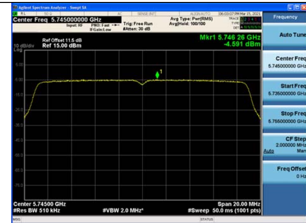
Test Mode:802. 11ac VHT20 Ant7
