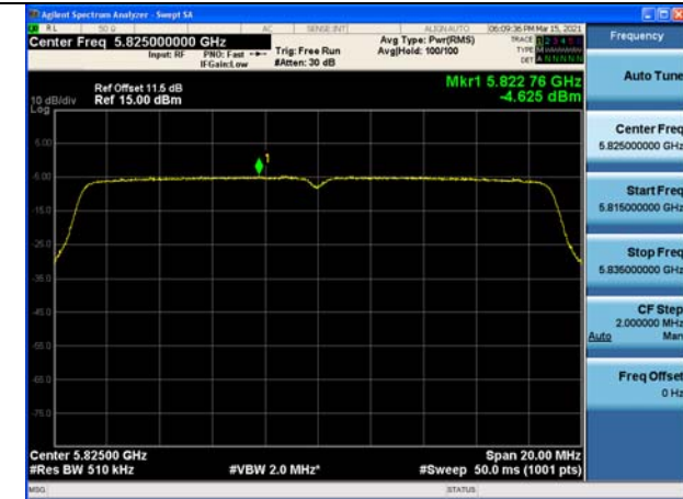
Test Mode:802. 11ac VHT20 Ant8
