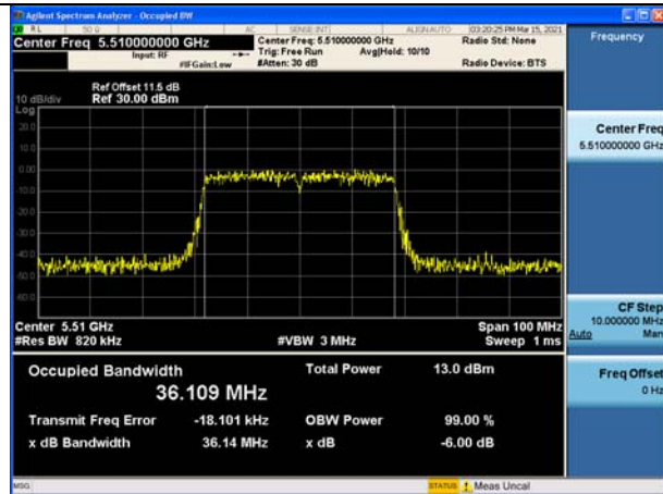
Test Mode:802. 11n HT40 Ant8
