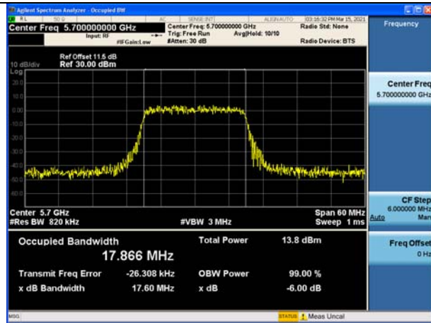
Test Mode:802. 11n HT20 Ant8
