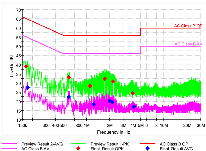
Pic3. Conducted emission L&N Line
