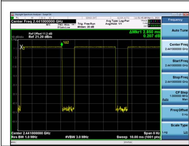
Modulation: GFSK DH5 2441
