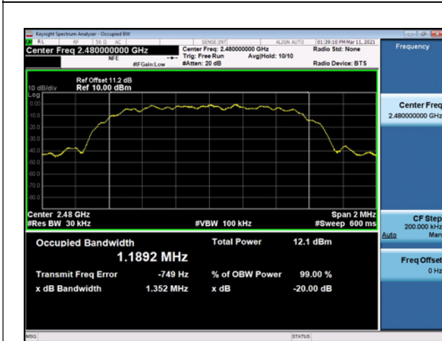
Modulation: 8DPSK 2480MHz
