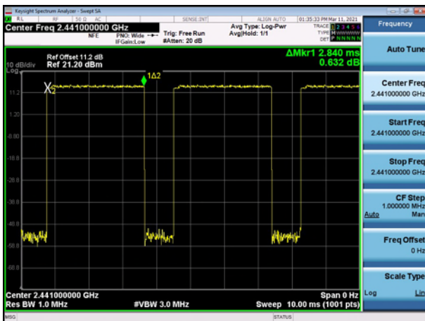
Modulation: 8DPSK DH5 2441
