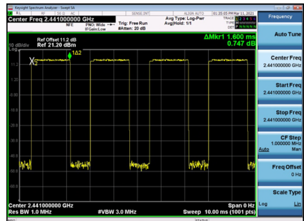
Modulation: 8DPSK DH3 2441
