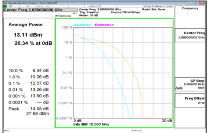
LTE_Band41_10MHz_64QAM_50_0_HighCH41540-2685
