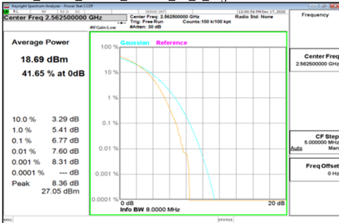
LTE_Band7_15MHz_64QAM_75_0_HighCH21375-2562.5
