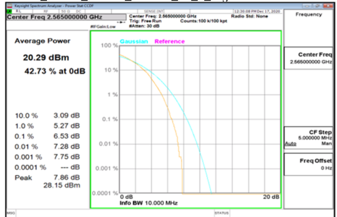
LTE_Band7_10MHz_64QAM_50_0_HighCH21400-2565
