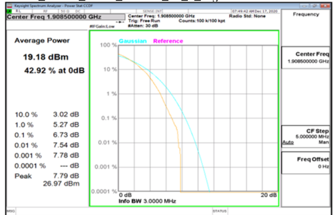
LTE_Band2_3MHz_64QAM_15_0_HighCH19185-1908.5
