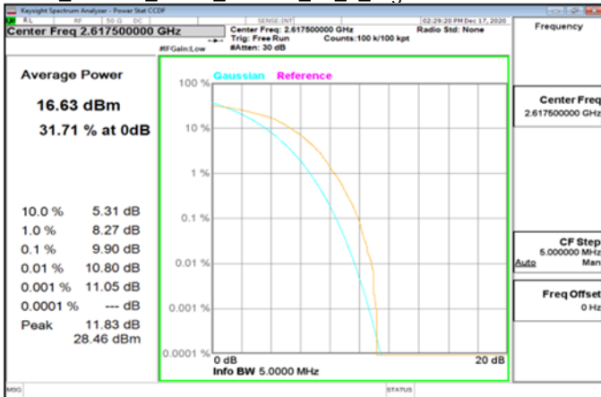
LTE_Band38_5MHz_64QAM_25_0_HighCH38225-2617.5
