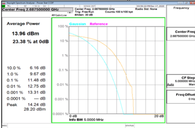
LTE_Band41_5MHz_64QAM_25_0_HighCH41565-2687.5
