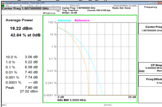
LTE_Band2_5MHz_64QAM_25_0_HighCH19175-1907.5
