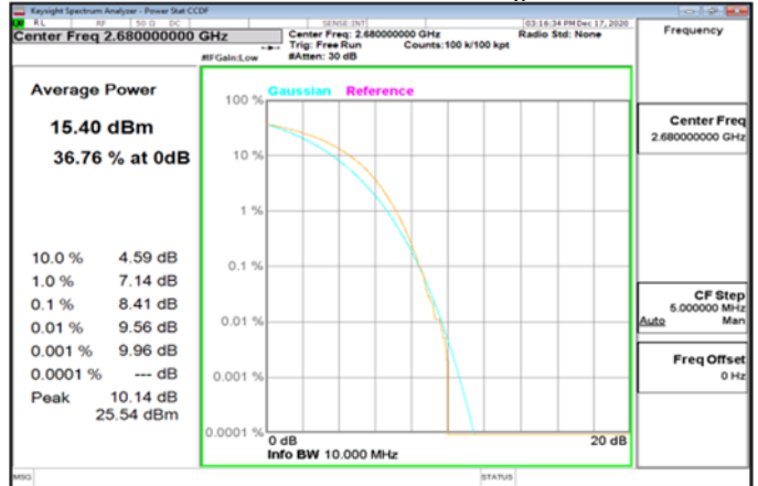
LTE_Band41_20MHz_64QAM_100_0_HighCH41490-2680
