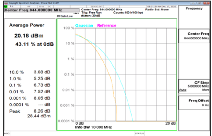
LTE_Band5_10MHz_64QAM_50_0_HighCH20600-844
