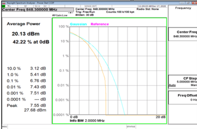
LTE_Band5_1_4MHz_64QAM_6_0_HighCH20643-848.3
