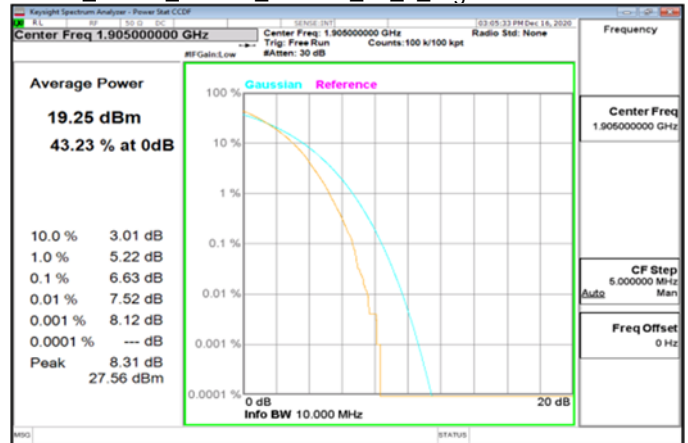
LTE_Band2_10MHz_64QAM_50_0_HighCH19150-1905
