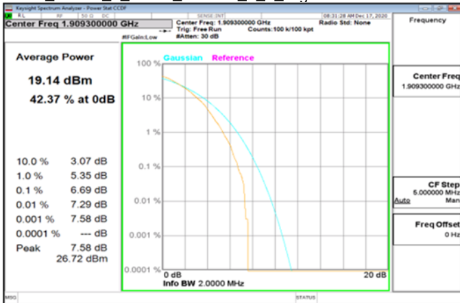
LTE_Band2_1_4MHz_64QAM_6_0_HighCH19193-1909.3
