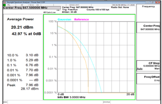
LTE_Band5_3MHz_64QAM_15_0_HighCH20635-847.5
