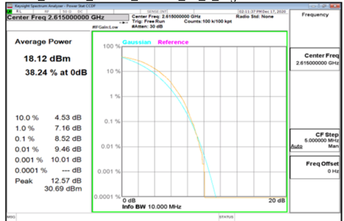
LTE_Band38_10MHz_64QAM_50_0_HighCH38200-2615
