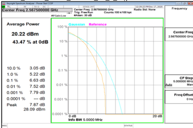
LTE_Band7_5MHz_64QAM_25_0_HighCH21425-2567.5
