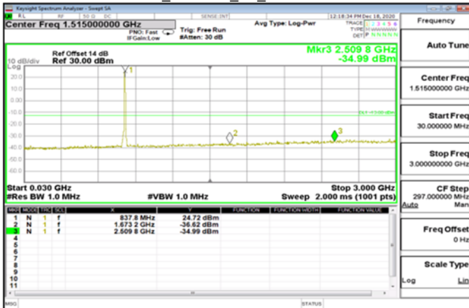
30MHz~3GHz_WCDMA_B5_MidCH4183-836.6
