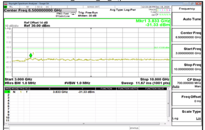
3GHz-10GHz_HSUPA_B5_HighCH4233-846.6
