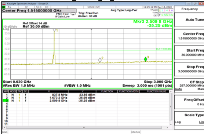
30MHz-3GHz_HSDPA_B5_MidCH4183-836.6
