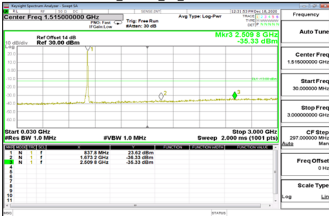
30MHz-3GHz_HSUPA_B5_MidCH4183-836.6
