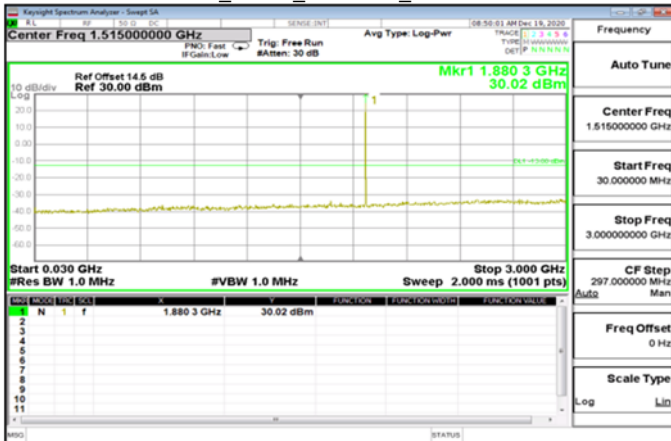
30MHz-3GHz_GPRS_1900MHz_MidCH661-1880
