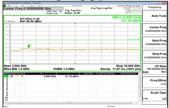
3GHz~10GHz_WCDMA_B5_HighCH4233-846.6
