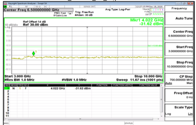
3GHz-10GHz_HSDPA_B5_HighCH4233-846.6
