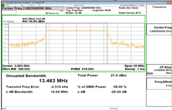
Band41_15MHz_64QAM_75_0_Main_HighCH41515-2682.5
