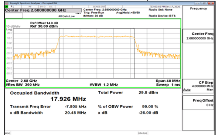
Band41_20MHz_QPSK_100_0_Main_HighCH41490-2680
