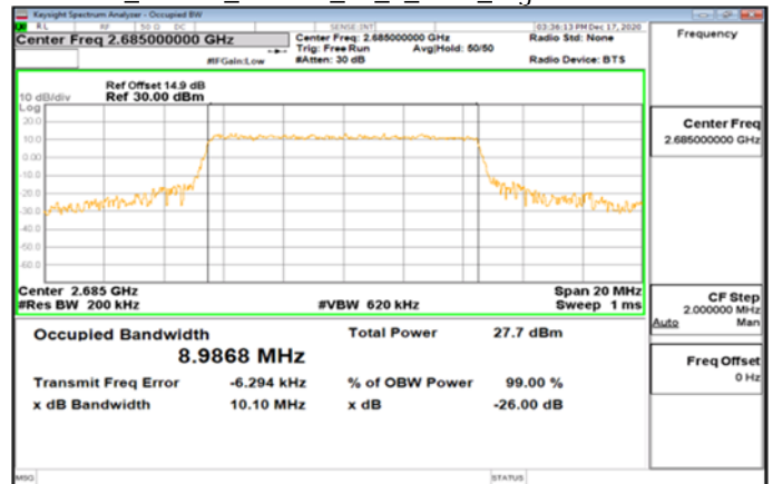
Band41_10MHz_64QAM_50_0_Main_HighCH41540-2685
