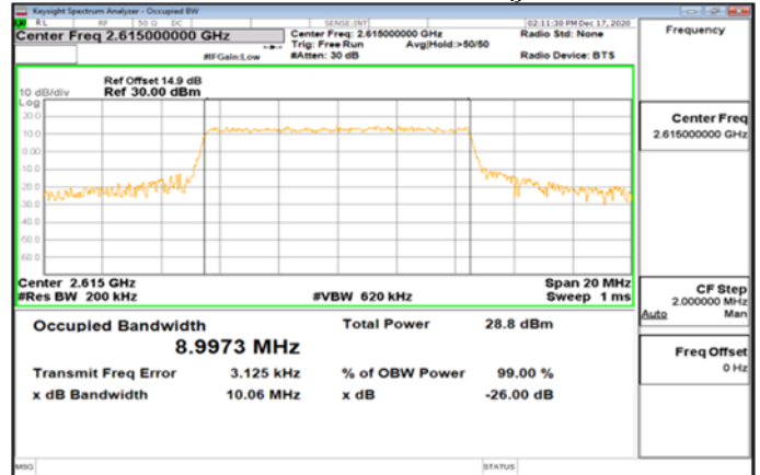
Band38_10MHz_64QAM_50_0_Main_HighCH38200-2615
