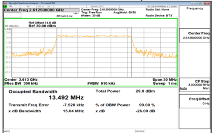
Band38_15MHz_16QAM_75_0_Main_HighCH38175-2612.5
