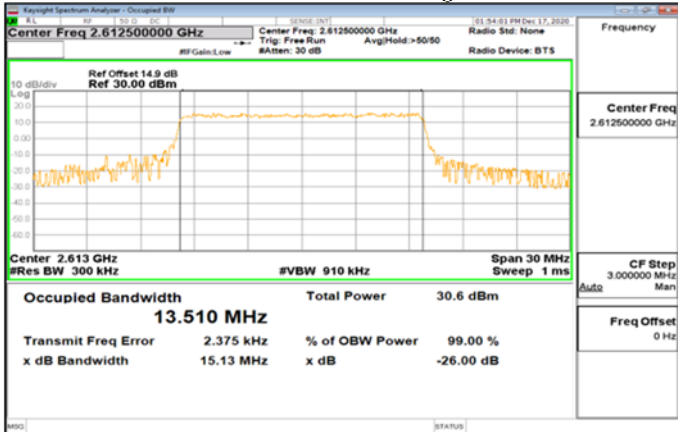
Band38_15MHz_QPSK_75_0_Main_HighCH38175-2612.5
