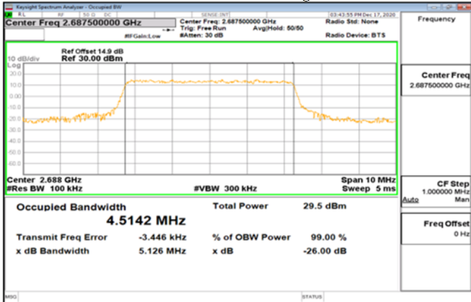
Band41_5MHz_QPSK_25_0_Main_HighCH41565-2687.5
