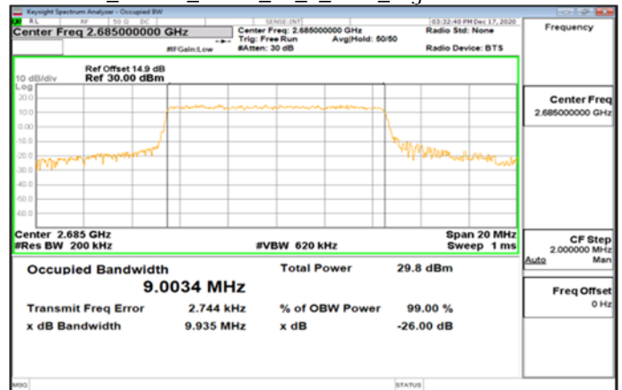
Band41_10MHz_QPSK_50_0_Main_HighCH41540-2685
