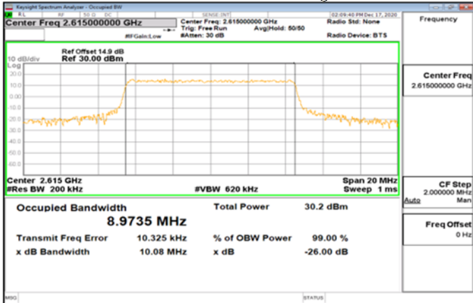
Band38_10MHz_16QAM_50_0_Main_HighCH38200-2615
