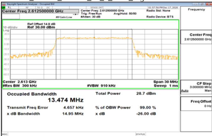
Band38_15MHz_64QAM_75_0_Main_HighCH38175-2612.5
