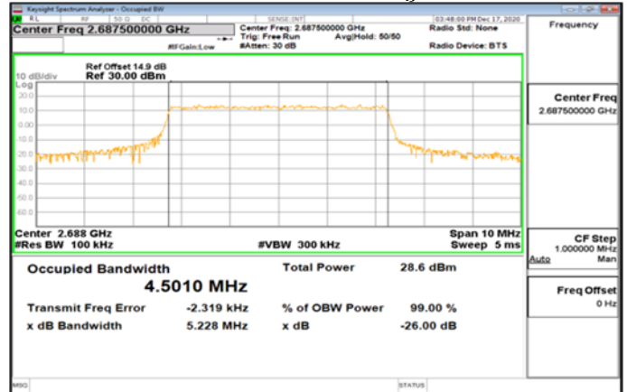
Band41_5MHz_16QAM_25_0_Main_HighCH41565-2687.5
