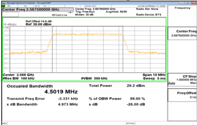
Band7_5MHz_64QAM_25_0_Main_HighCH21425-2567.5
