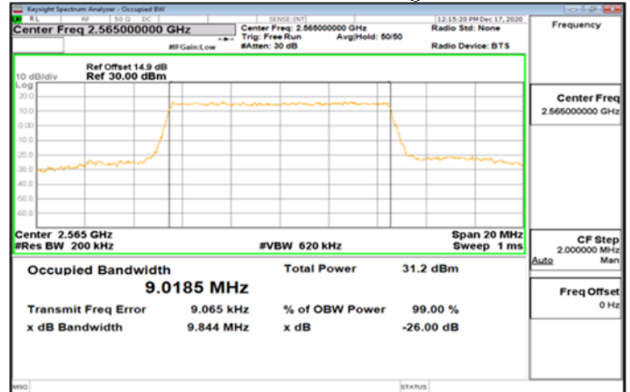
Band7_10MHz_QPSK_50_0_Main_HighCH21400-2565
