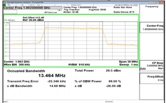
Band2_15MHz_16QAM_75_0_Main_HighCH19125-1902.5
