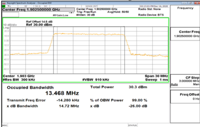
Band2_15MHz_QPSK_75_0_Main_HighCH19125-1902.5
