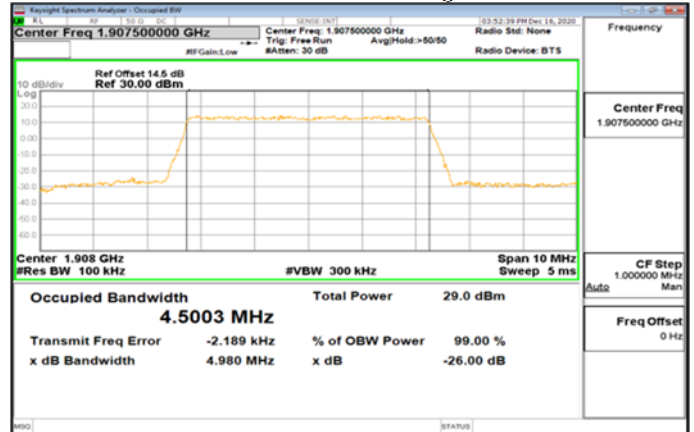
Band2_5MHz_16QAM_25_0_Main_HighCH19175-1907.5
