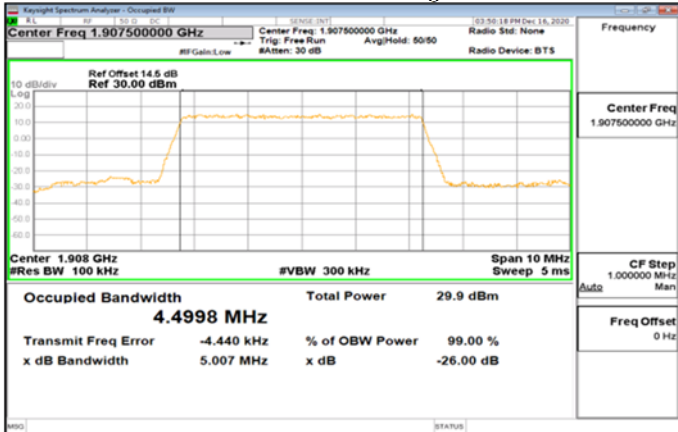
Band2_5MHz_QPSK_25_0_Main_HighCH19175-1907.5
