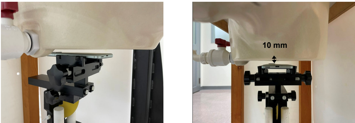
Fig.10 EUT Back side to flat phantom
