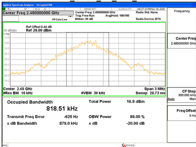
OBW 20dB_GFSK_1M_DH5_2480MHz
