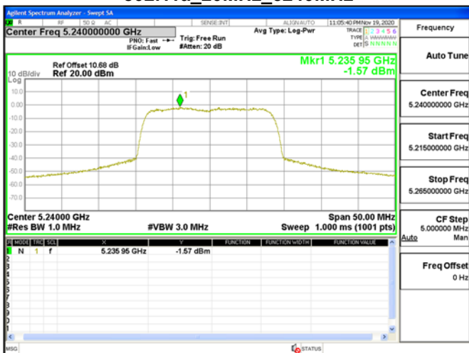
802.11a_20MHz_5240MHz
