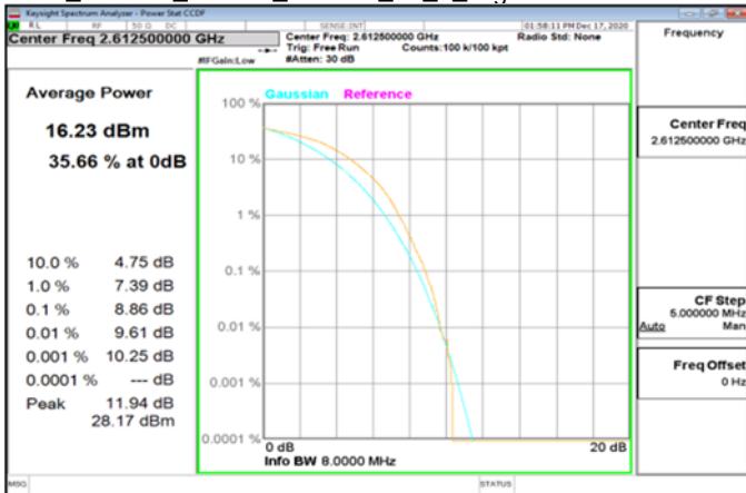
LTE_Band38_15MHz_64QAM_75_0_HighCH38175-2612.5
