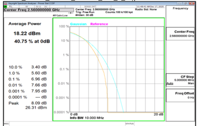
LTE_Band7_20MHz_64QAM_100_0_HighCH21350-2560
