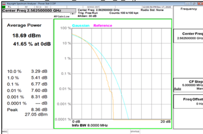
LTE_Band7_15MHz_64QAM_75_0_HighCH21375-2562.5
