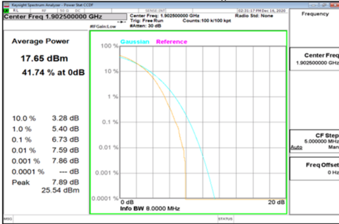
LTE_Band2_15MHz_64QAM_75_0_HighCH19125-1902.5
