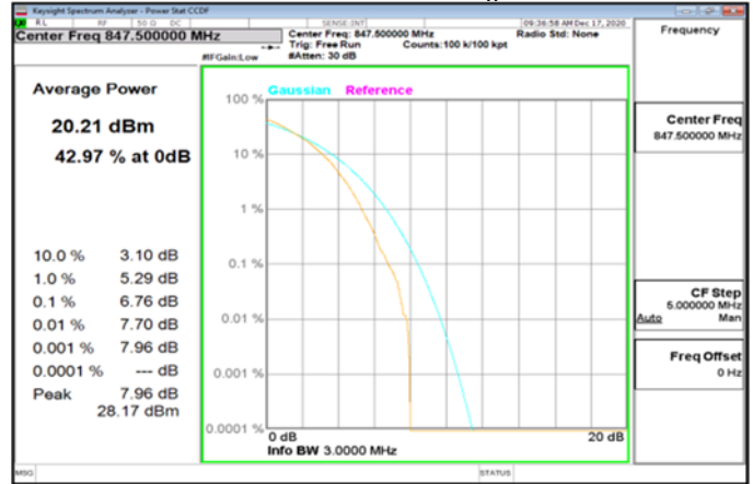
LTE_Band5_3MHz_64QAM_15_0_HighCH20635-847.5
