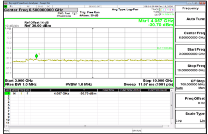
3GHz~10GHz_GSM_850MHz_HighCH251-848.8
