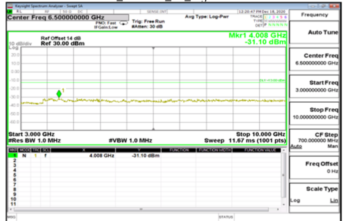
3GHz~10GHz_WCDMA_B5_HighCH4233-846.6
