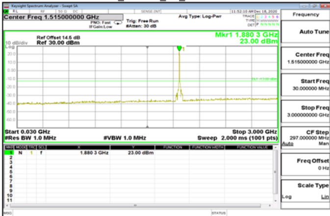
30MHz~3GHz_HSDPA_B2_MidCH9400-1880
