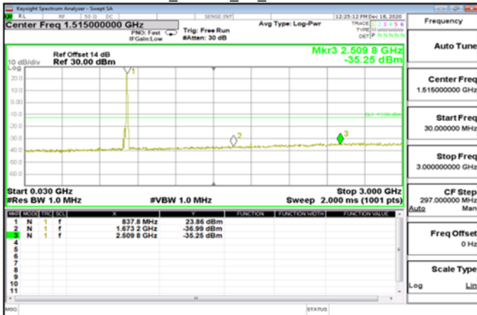
30MHz-3GHz_HSDPA_B5_MidCH4183-836.6
