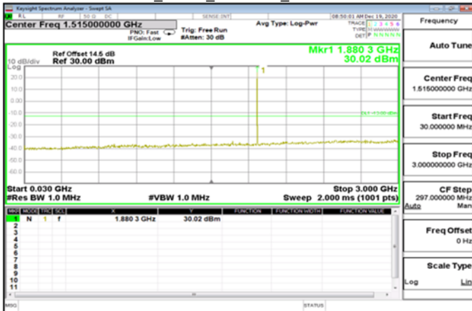
30MHz-3GHz_GPRS_1900MHz_MidCH661-1880
