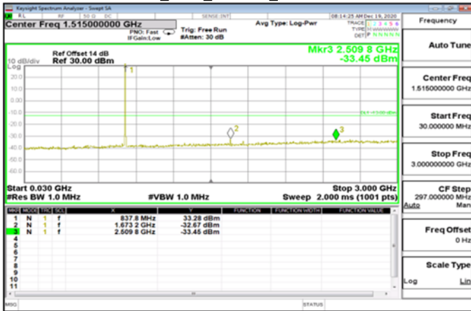
30MHz~3GHz_GSM_850MHz_MidCH190-836.6
