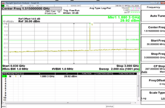
30MHz~3GHz_GSM_1900MHz_MidCH661-1880
