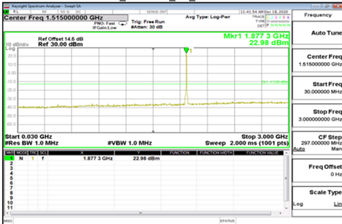
30MHz~3GHz_WCDMA_B2_MidCH9400-1880
