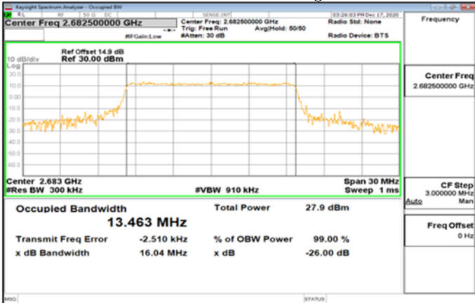
Band41_15MHz_64QAM_75_0_Main_HighCH41515-2682.5
