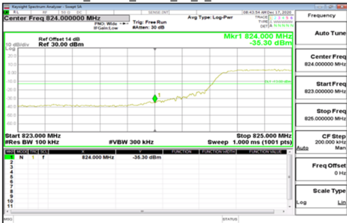
LTE\Band5_10MHz_QPSK_50_0_LowCH20450-829
