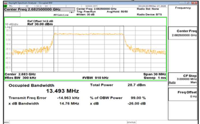
Band41_15MHz_16QAM_75_0_Main_HighCH41515-2682.5
