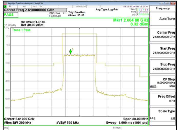
Band38_20MHz\QPSK_RB100_0_CH38150
