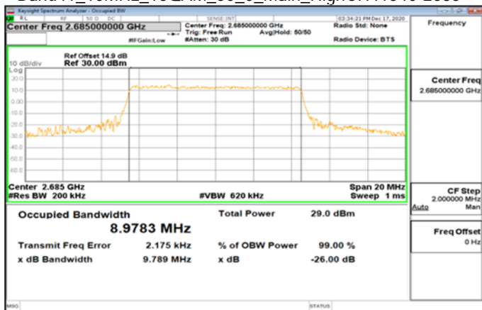
Band41_10MHz_16QAM_50_0_Main_HighCH41540-2685
