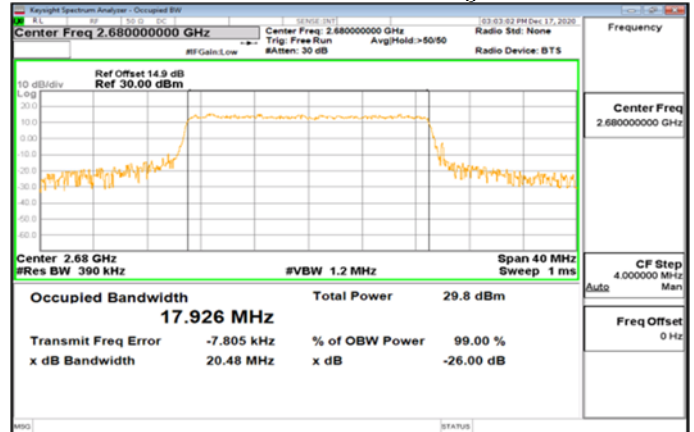
Band41_20MHz_QPSK_100_0_Main_HighCH41490-2680
