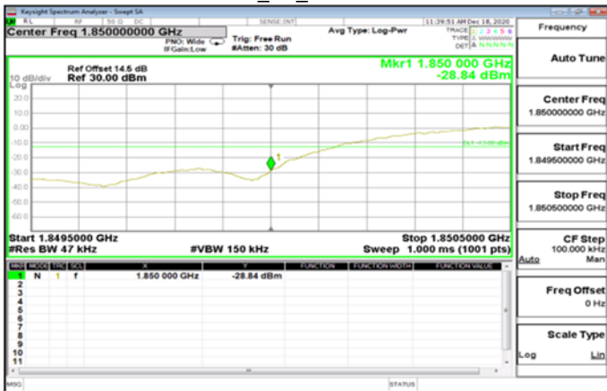
WCDMA\WCDMA_B2_LowCH9262-1852.4
