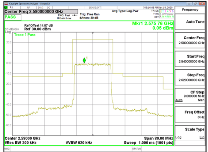
Band38_20MHz\QPSK_RB100_0_CH38150
