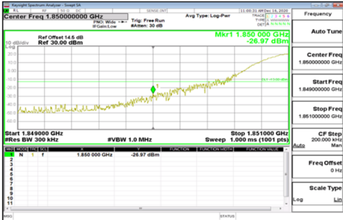
LTE\Band2_20MHz_QPSK_1_0_LowCH18700-1860
