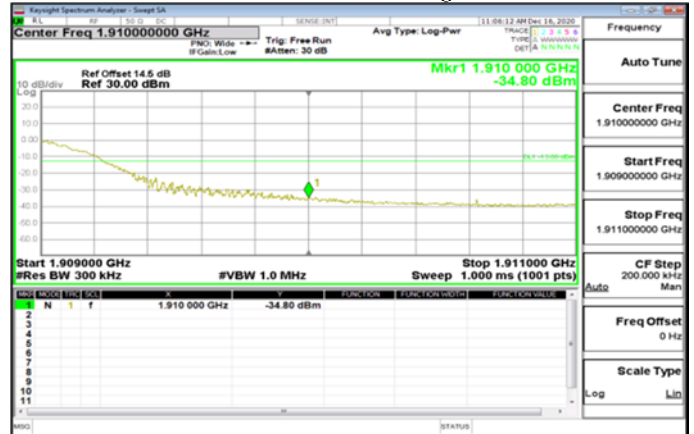
LTE\Band2_20MHz_QPSK_100_0_HighCH19100-1900
