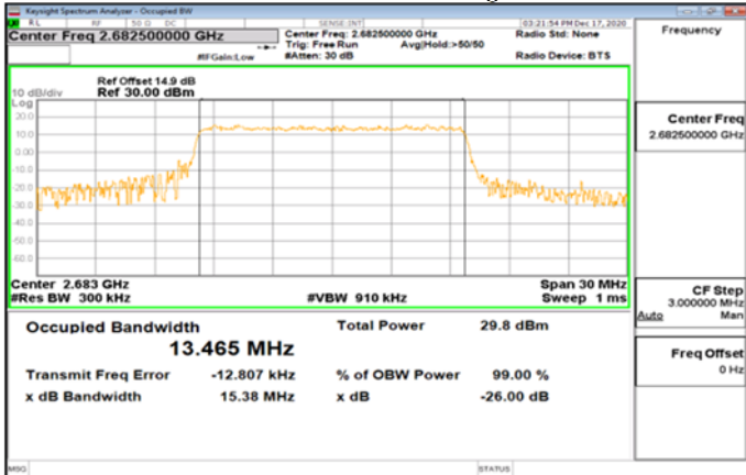
Band41_15MHz_QPSK_75_0_Main_HighCH41515-2682.5
