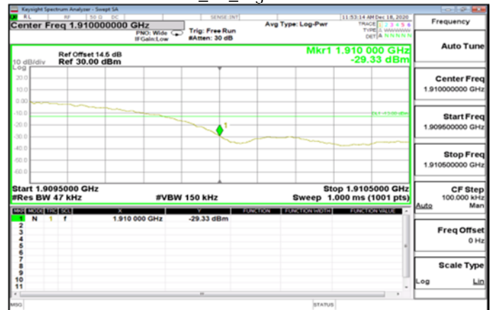
HSDPA\HSDPA_B2_HighCH9538-1907.6
