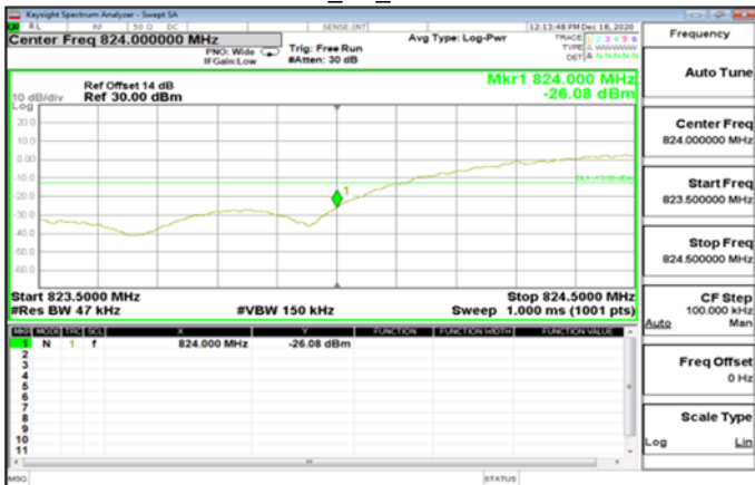
WCDMAWCDMA_B5_LowCH4132-826.4
