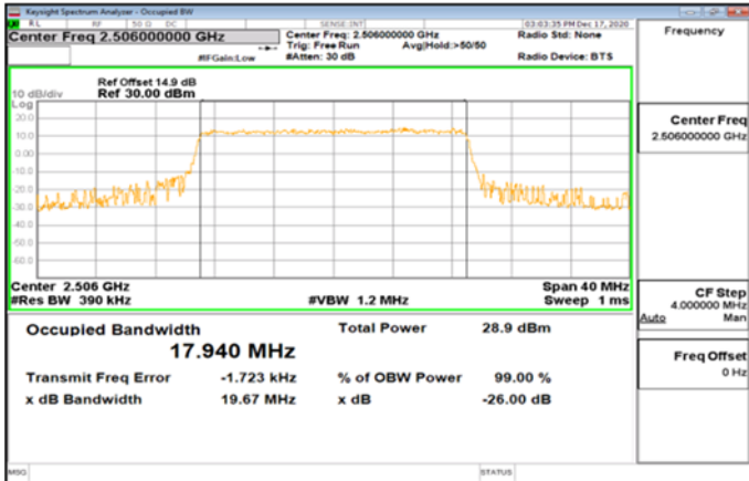
Band41_20MHz_16QAM_100_0_Main_MidCH40620-2593
