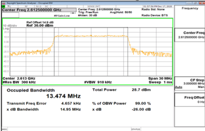
Band38_15MHz_64QAM_75_0_Main_HighCH38175-2612.5
