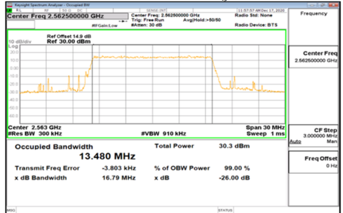
Band7_15MHz_16QAM_75_0_Main_HighCH21375-2562.5
