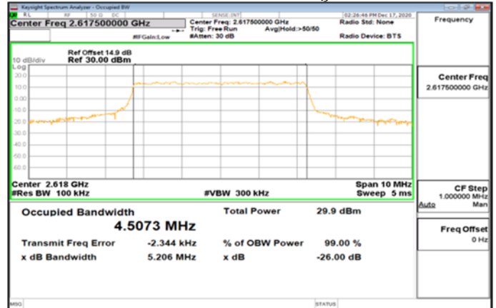
Band38_5MHz_16QAM_25_0_Main_HighCH38225-2617.5
