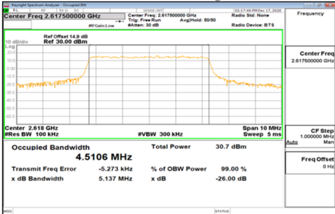
Band38_5MHz_QPSK_25_0_Main_HighCH38225-2617.5
