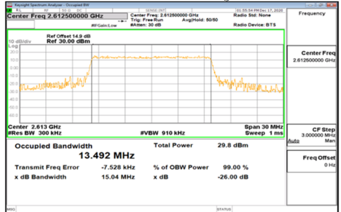
Band38_15MHz_16QAM_75_0_Main_HighCH38175-2612.5
