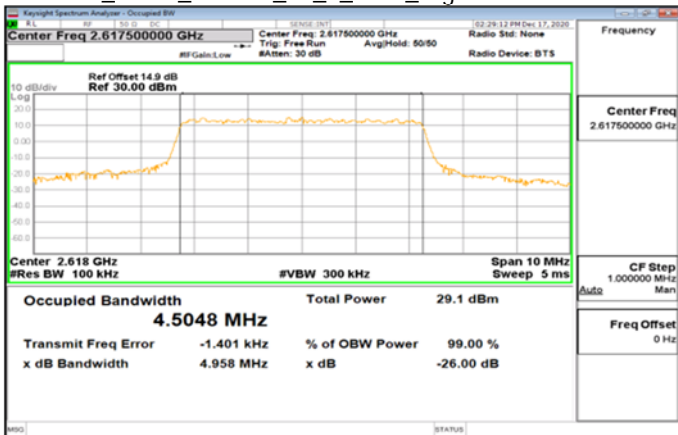
Band38_5MHz_64QAM_25_0_Main_HighCH38225-2617.5
