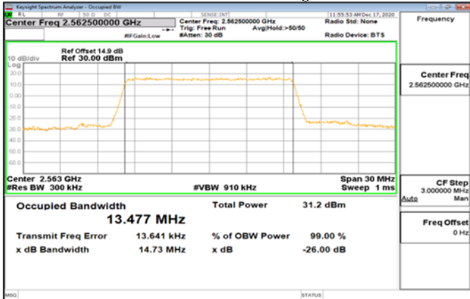
Band7_15MHz_QPSK_75_0_Main_HighCH21375-2562.5
