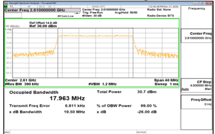
Band38_20MHz_QPSK_100_0_Main_HighCH38150-2610
