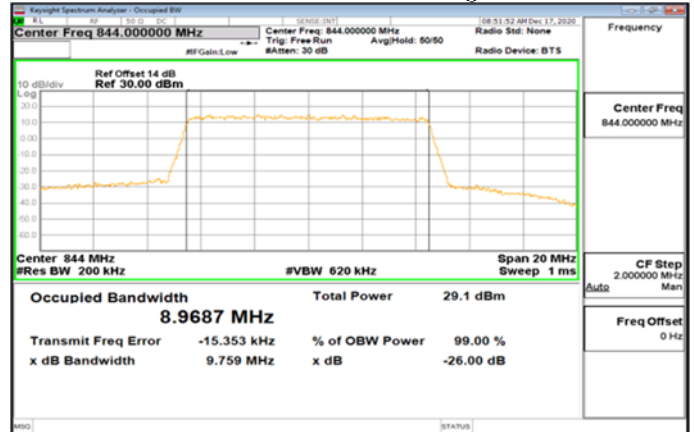
Band5_10MHz_64QAM_50_0_Main_HighCH20600-844
