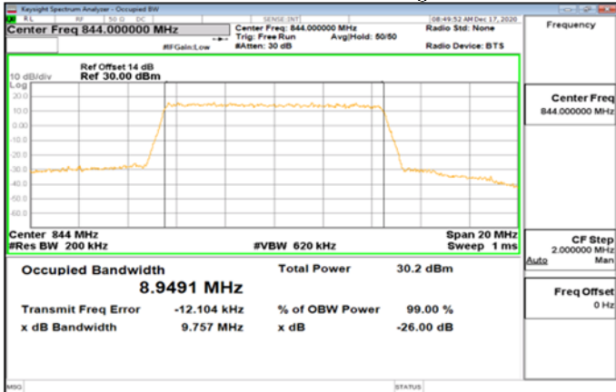
Band5_10MHz_16QAM_50_0_Main_HighCH20600-844
