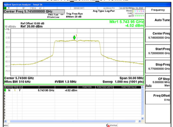
802.11a_20MHz_5745MHz
