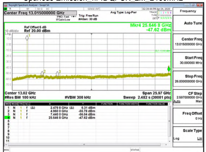
Spurious Emission_π/4QPSK_2M_2480MHz
