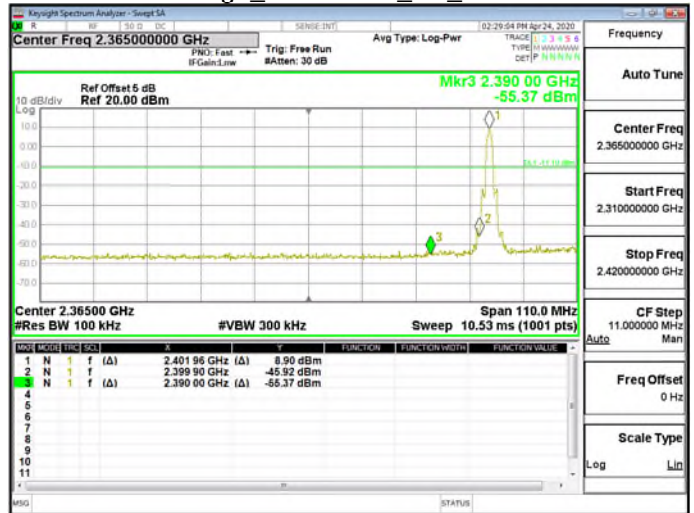
Hopping Band Edge_pi/4QPSK_2M_2402MHz
