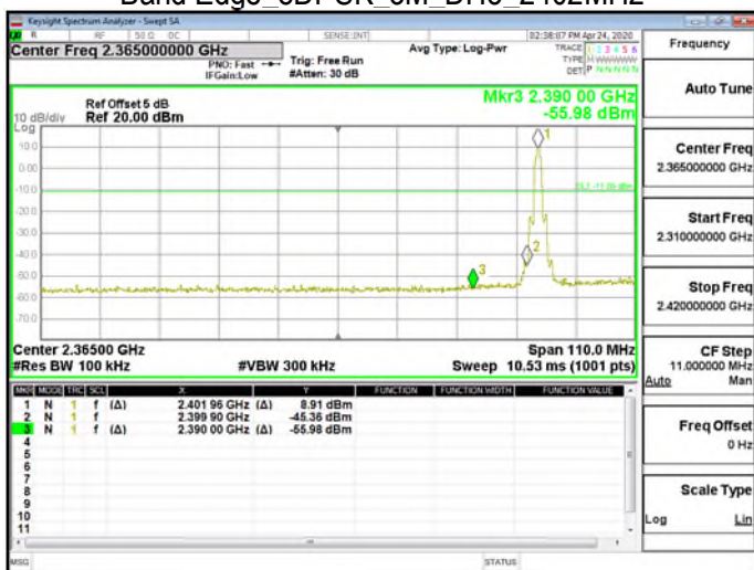
Band Edge_8DPSK_3M_DH5_2402MHz
