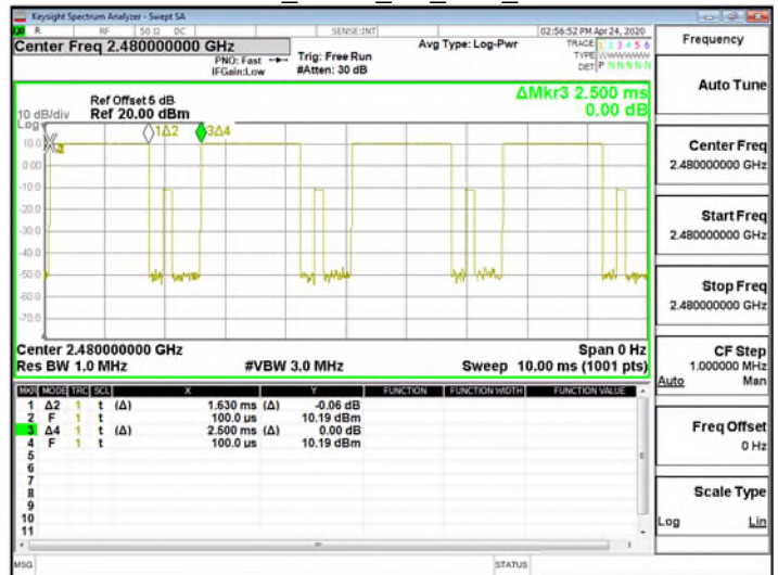
Dwell Time_GFSK_1M_DH3_2480MHz
