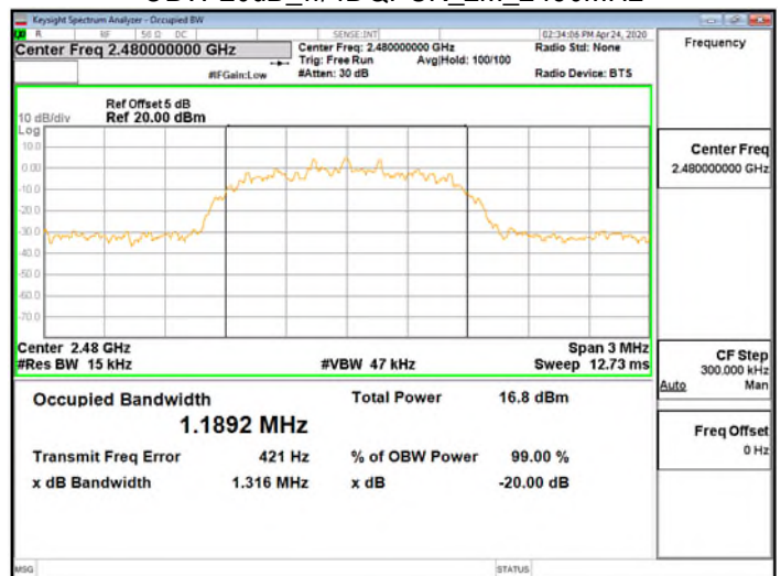
OBW 20dB_π/4DQPSK_2M_2480MHz
