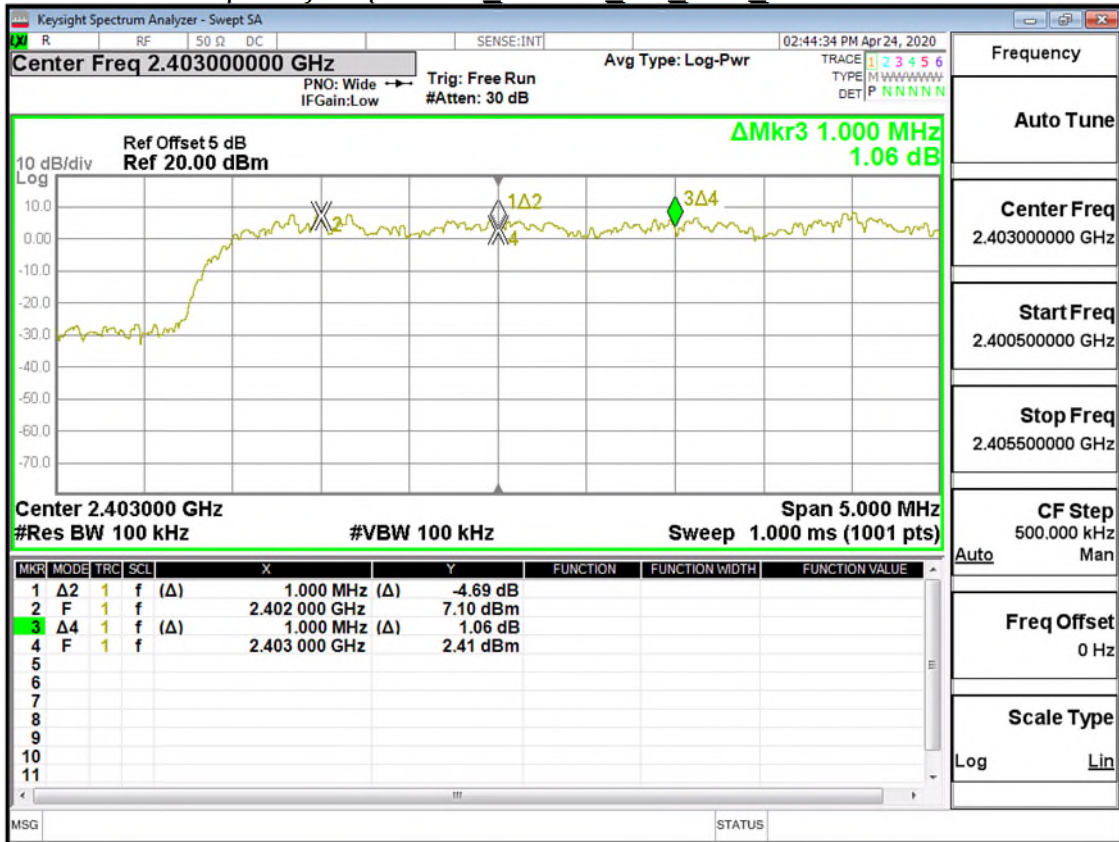
Frequency Separation_8DPSK_3M_DH5_CH0CH1CH2
