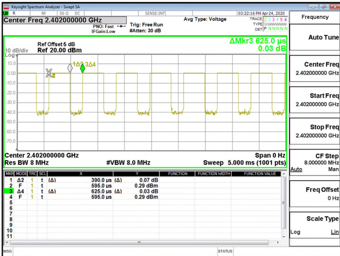
Duty Cycle_BLE_1M_LowCH00-2402
