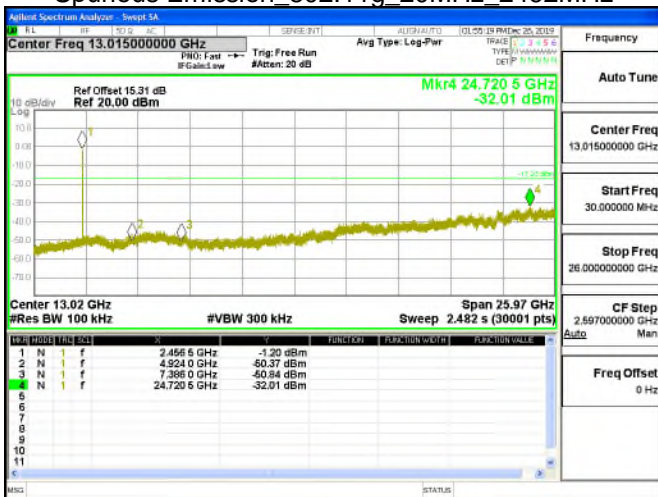
Spurious Emission_802.11g_20MHz_2462MHz
