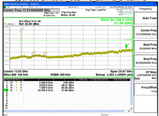
Spurious Emission_802.11b_20MHz_2462MHz
