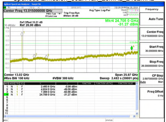
Spurious Emission_802.11ax_20MHz_2462MHz
