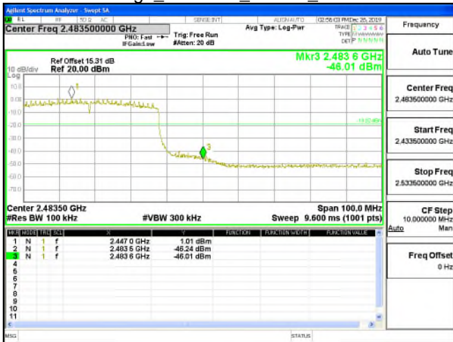
Band Edge_802.11ax_40MHz_2452MHz
