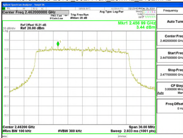
Reference Level_802.11ax_20MHz_2462MHz
