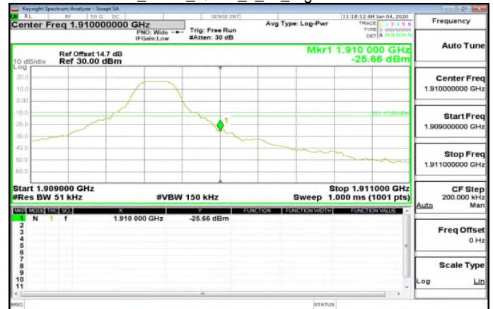
LTE\Band2_5MHz_QPSK_1_24_HighCH19175-1907.5
