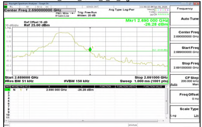
LTE\Band41_5MHz_QPSK_1_24_HighCH41565-2687.5
