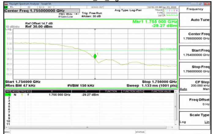
HSDPA\HSDPA_B4_HighCH1513-1752.6
