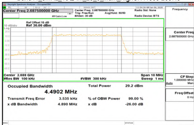
Band41_5MHz_16QAM_25_0_Main_HighCH41565-2687.5
