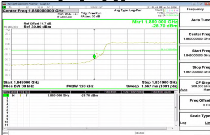
LTE\Band2_3MHz_QPSK_15_0_LowCH18615-1851.5
