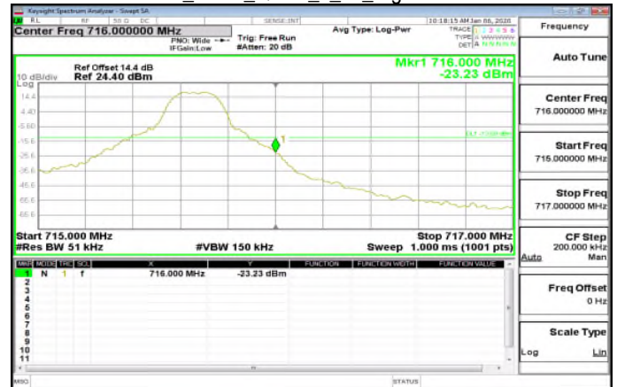
LTE\Band17_5MHz_QPSK_1_24_HighCH23825-713.5
