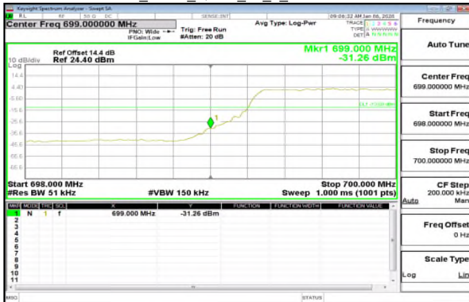
LTE\Band12_5MHz_QPSK_25_0_LowCH23035-701.5
