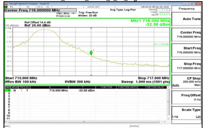
LTE\Band12_10MHz_QPSK_1_49_HighCH23130-711
