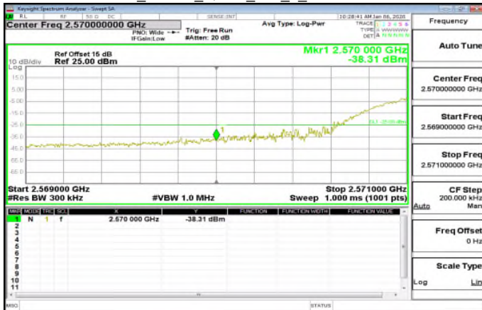
LTE\Band38_20MHz_QPSK_100_0_LowCH37850-2580
