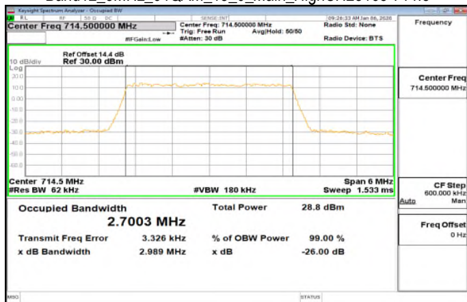
Band12_3MHz_64QAM_15_0_Main_HighCH23165-714.5
