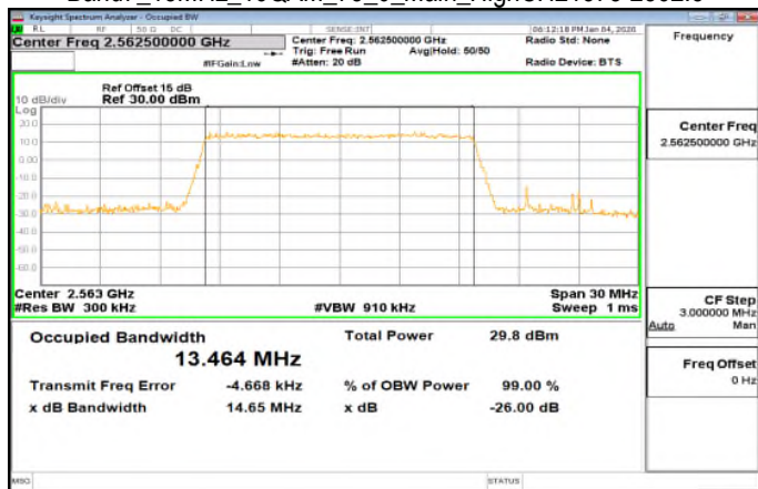
Band7_15MHz_16QAM_75_0_Main_HighCH21375-2562.5
