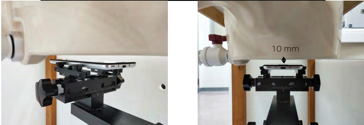
Fig.9 EUT Front side to flat phantom
