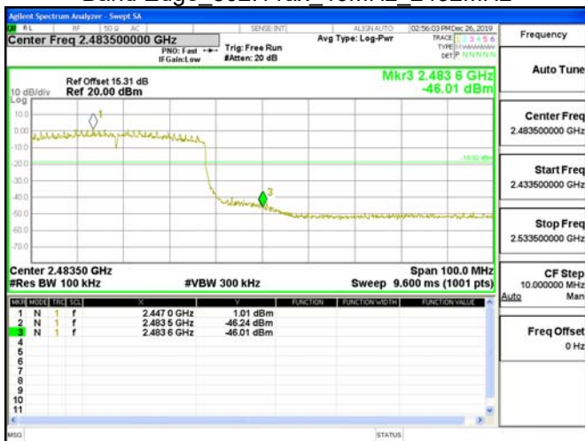
Band Edge 802.11ax 40MHz 2452MHz
