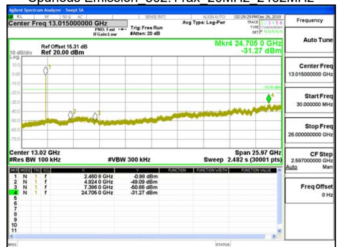
Spurious Emission 802.11ax 20MHz 2462MHz
