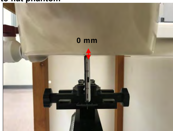
Fig.17 EUT Right side to flat phantom
