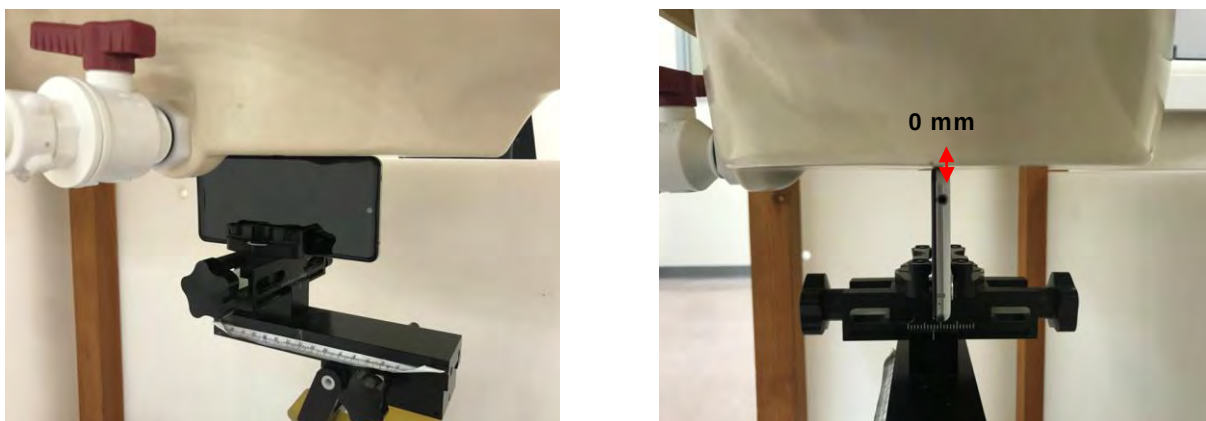
Fig.19 EUT Left side to flat phantom
