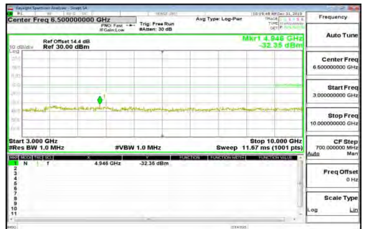
3GHz-10GHz_Band12_5MHz_QPSK_1_0_MidCH23095-707.5
