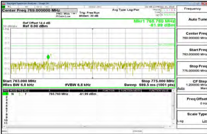
Inband-2_Band13_5MHz_QPSK_1_0_MidCH23230-782
