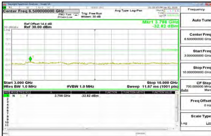
3GHz-10GHz_GSM_850MHz_LowCH128-824.2
