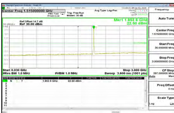
30MHz-3GHz_WCDMA_B2_LowCH9262-1852.4
