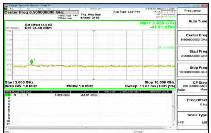
3GHz-10GHz_Band12_10MHz_QPSK_1_0_MidCH23095-707.5
