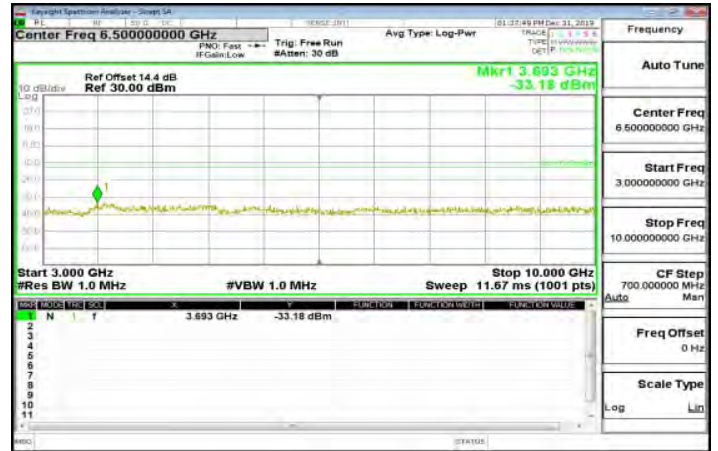
Inband-1_Band13_5MHz_QPSK_1_0_LowCH23205-779.5
