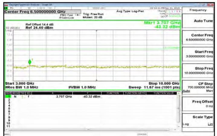
3GHz~10GHz_Band17_5MHz_QPSK_1_0_HighCH23825-713.5
