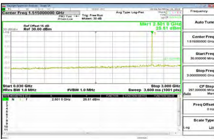
30MHz~3GHz_Band7_10MHz_QPSK_1_0_LowCH20800-2505
