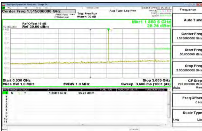
30MHz-3GHz_Band2_1_4MHz_QPSK_1_0_LowCH18607-1850.7
